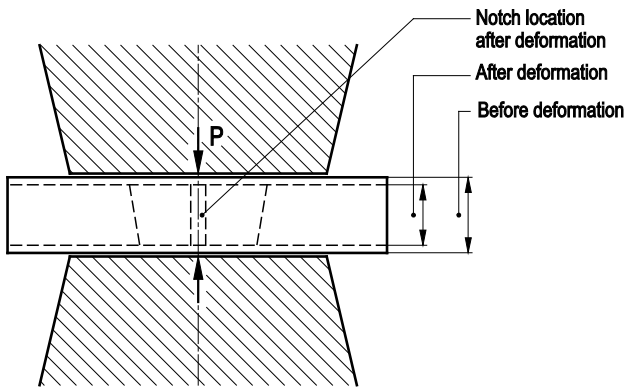
Figure 4.5.5-1: Upsetting of notched bar impact test specimens to be aged
