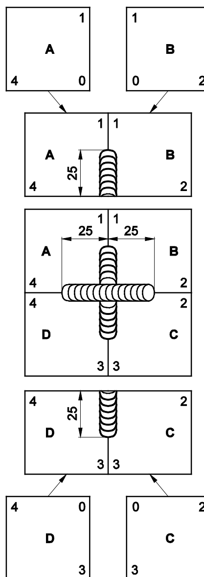
Figure E-2: Preparation of test coupon
