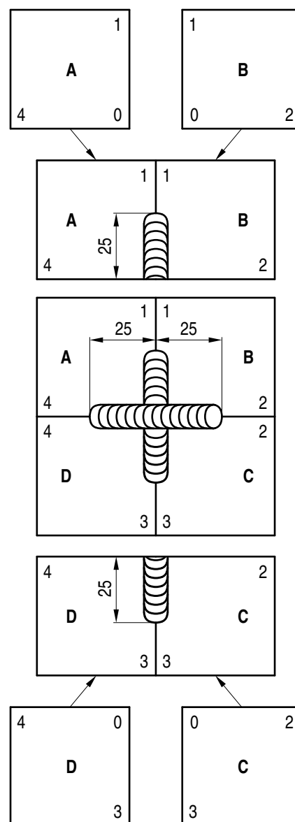
Figure B-2: Preparation of test coupon
