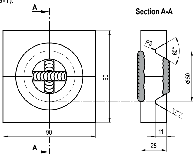
Figure B-1: Test coupon form
