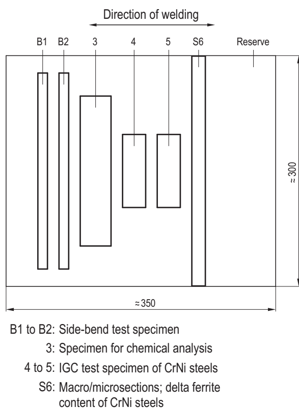
Figure 4-2: Test specimen location (schematic) in the test coupon for batch tests on weld filler metals for weld claddings of austenitic steels and nickel alloys
