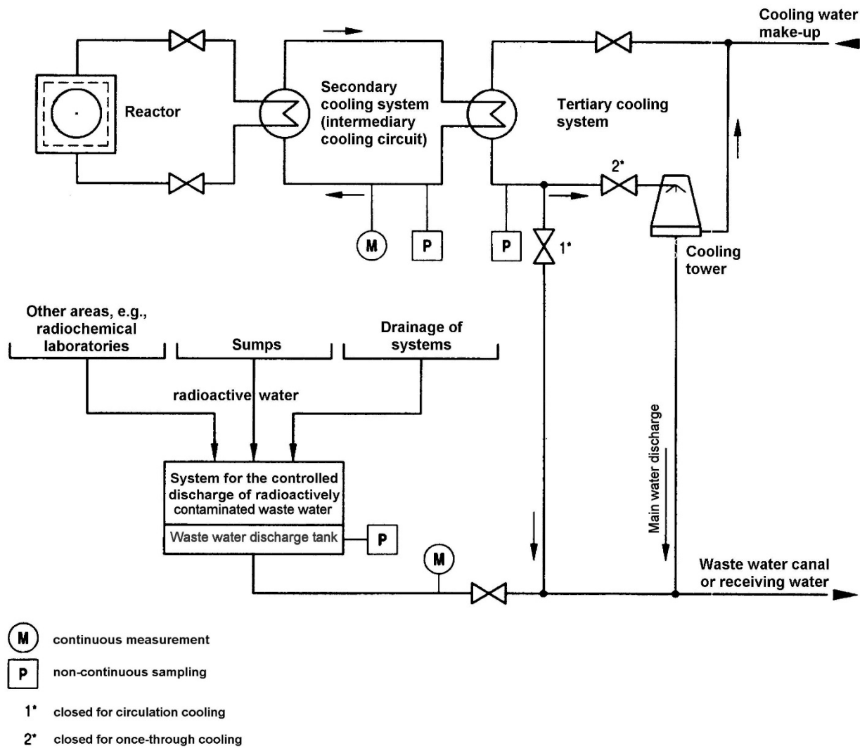
Figure 5-1: Monitoring of radioactive substances discharged with water; the example shown is a closed loop secondary cooling system
