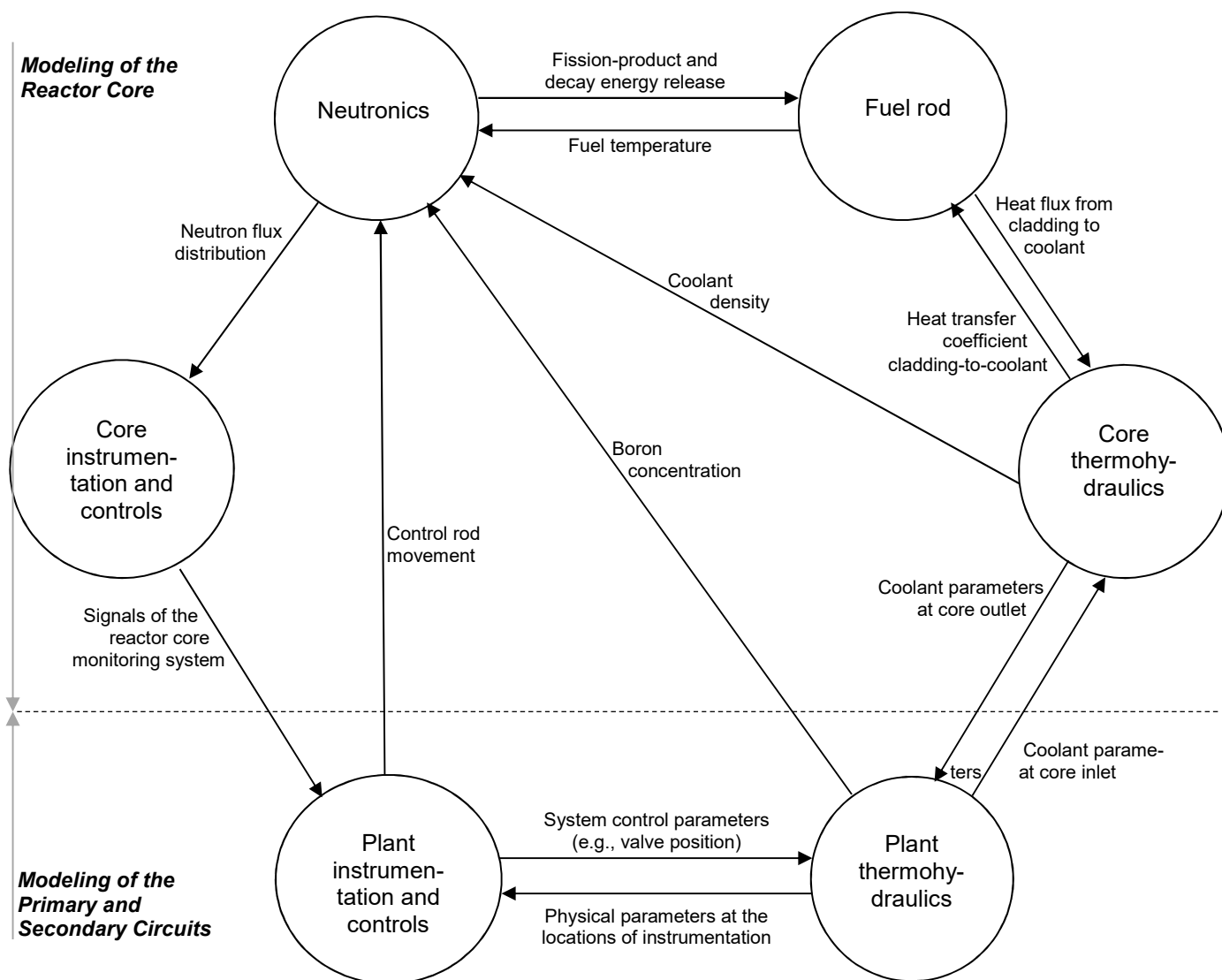
Figure 4-2: Example of a coupled program system
