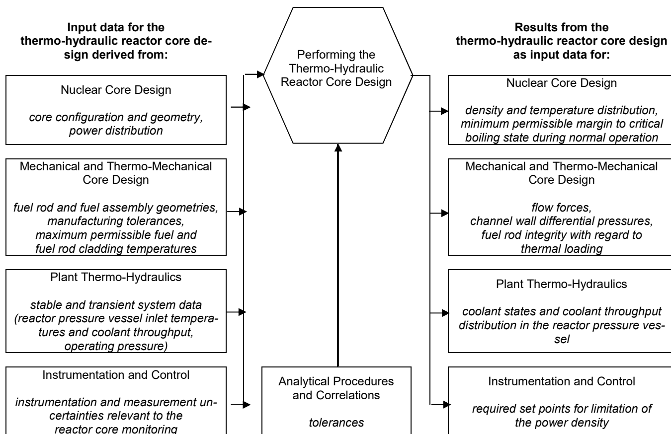
Figure 4-1: Interconnections of the thermo-hydraulic design of reactor cores with other analysis fields
