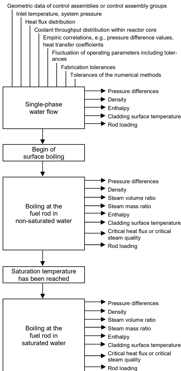
Figure 5-1: Requirements regarding treatment of the heat transfer to the coolant in the reactor cores of pressurized water and boiling water reactors
