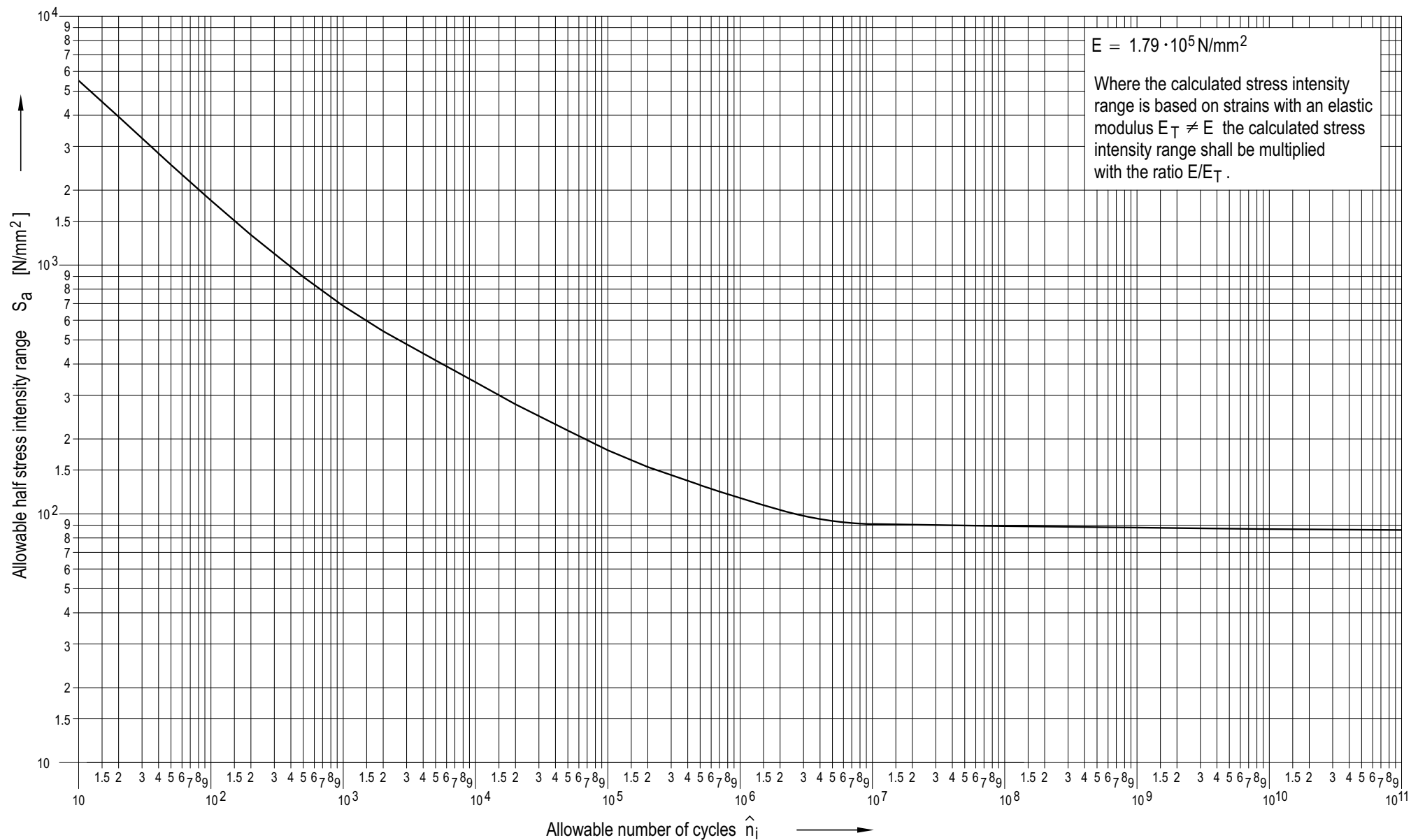
Figure B 5-3: Design fatigue curve for austenitic steels except the steels 1.4550 and 1.4541
