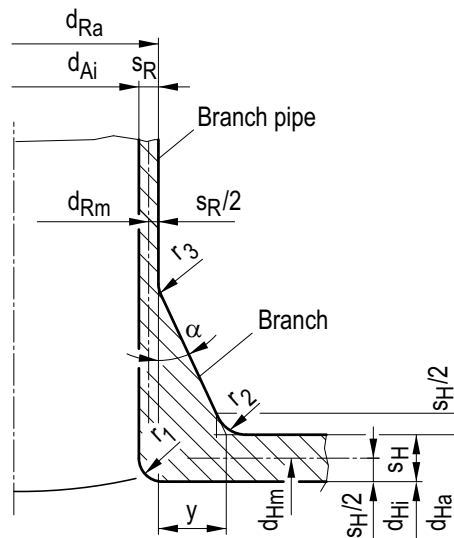
Figure A 4-13: Branch
