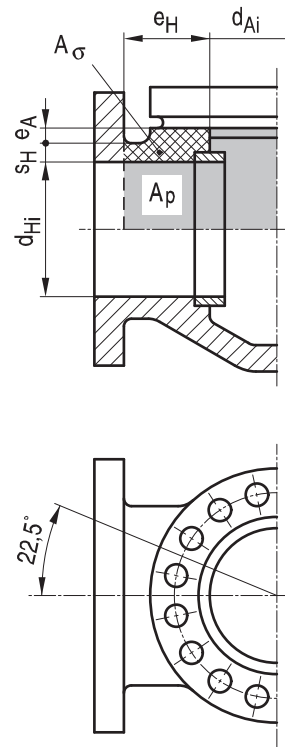
Figure A 3.1-7: Valve body
