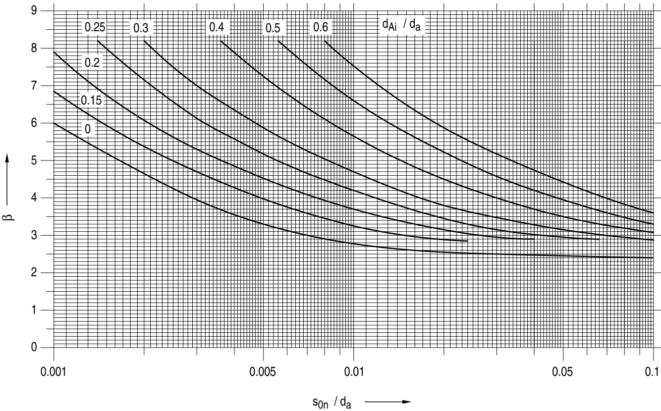
Figure A 2.5-3: Shape factors \beta for torispherical heads
