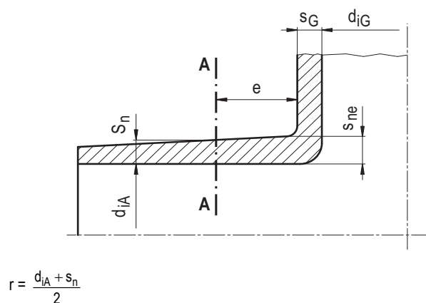
Figure 8.3-5: Critical section at conical valve bodies
