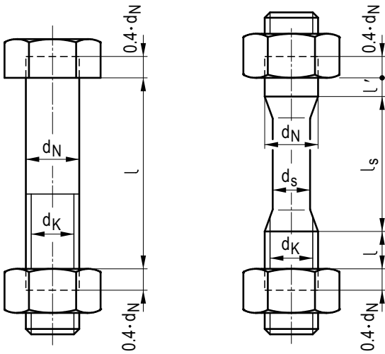
Full-shank bolt
