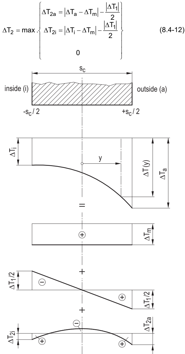
Figure 8.4-2: Decomposition of temperature distribution range
