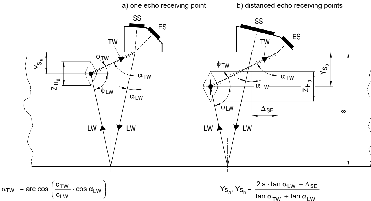
Figure C-17: Principle of LLT technique
