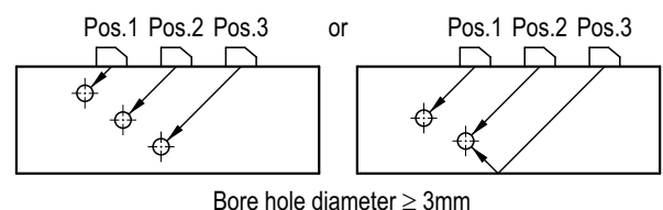
Figure C-2: Reference blocks for adjusting the testing level for angle beam scanning
