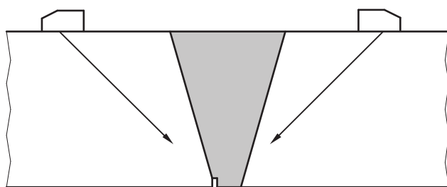
Figure 12-16: Location of notches and beam angles for the examination of welded joints on austenitic steels
