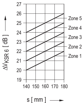
Wall thickness range (mm) 140 \leq s \leq 180 PK 1: 10 x 20 mm 2 , 2 MHz, 45 degrees PK 2: 20 x 22 mm 2 , 2 MHz, 45 degrees Edge zone allowance contained in \Delta V_{KSR6} : \Delta V_{Rand} = 5 \text{ dB}
