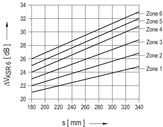
Wall thickness range (mm) 180 \leq s \leq 340 PK 1: 10 x 20 mm 2 , 2 MHz, 45 degrees PK 2: 20 x 22 mm 2 , 2 MHz, 45 degrees Edge zone allowance contained in \Delta V_{KSR6} : \Delta V_{Rand} = 5 \text{ dB}
