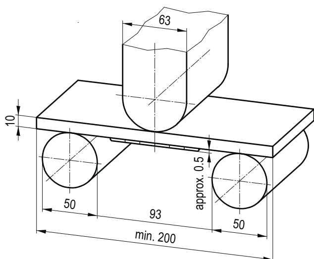
Specimen configuration and test geometry of side-bend test according to DIN EN ISO 5173.
