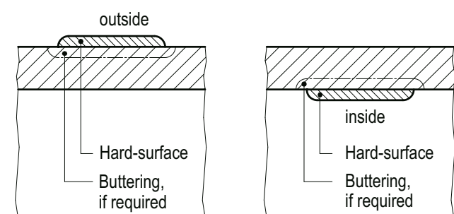
Figure 9-19: Hard surfacing on tubes
