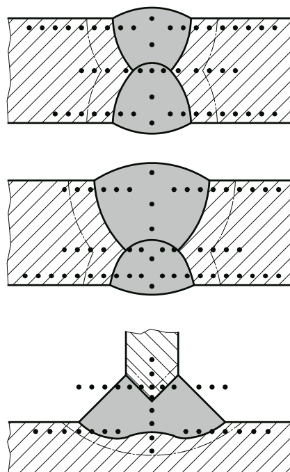
Examples of locations of hardness indentations
