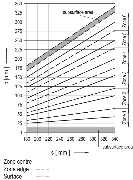
Wall thickness range (mm) 180 \leq s \leq 340 PK 1: 10 x 20 mm 2 , 2 MHz, 45 degrees PK 2: 20 x 22 mm 2 , 2 MHz, 45 degrees
