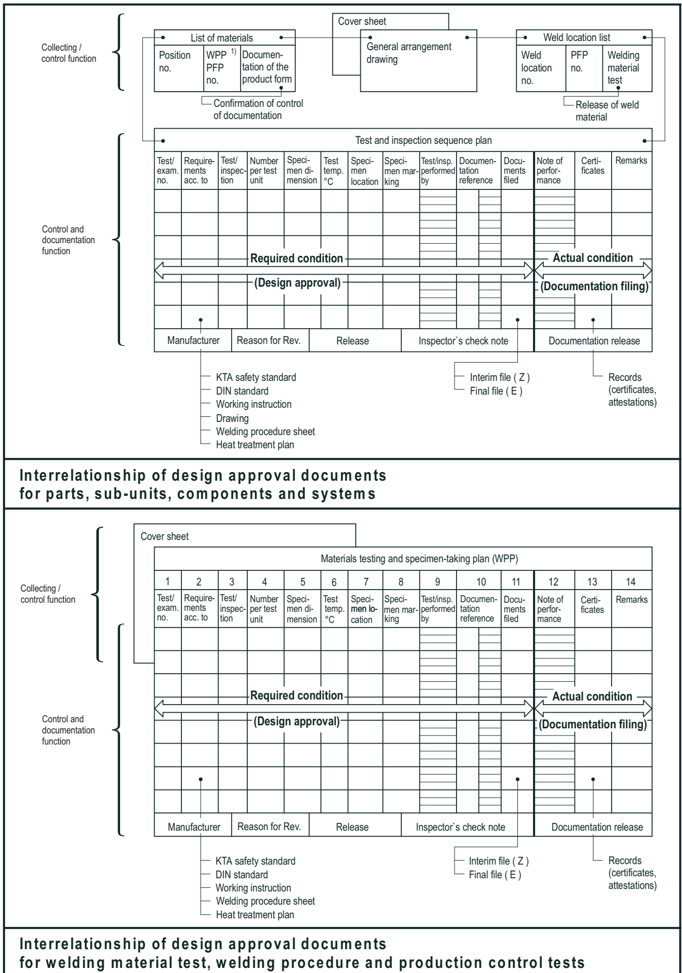
Figure 4-2: Interrelationship of design approval documents
