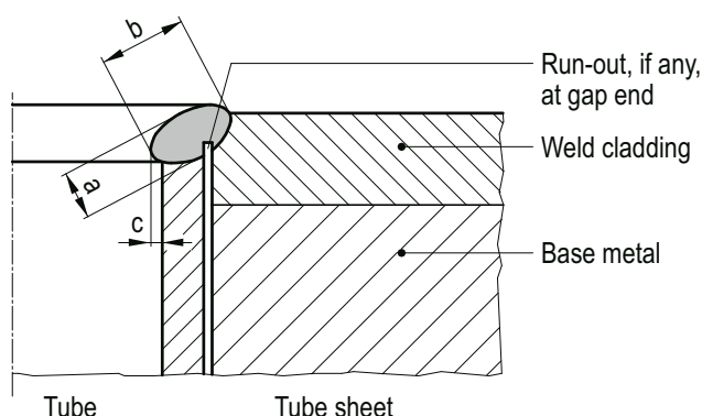
Figure 9-13: Tube-to-tubesheet weld
