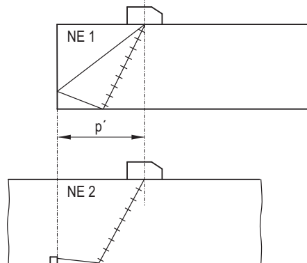
Figure C-15: Sound field geometry during transverse wave conversion
