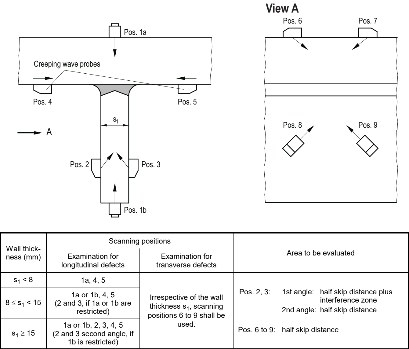
Figure 12-10: Scanning positions and number of beam angles for the examination of attachment welds (double bevel groove welds) as well as areas to be evaluated by angle beam scanning
