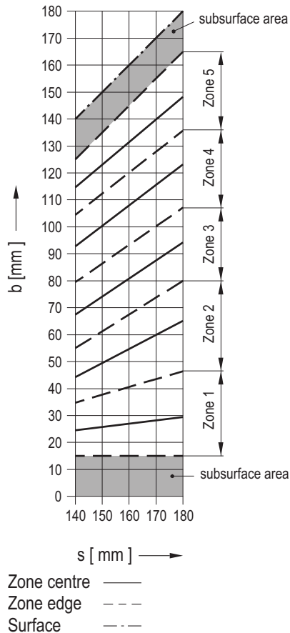
Wall thickness range (mm) 140 \leq s \leq 180 PK 1: 10 x 20 mm 2 , 2 MHz, 45 degrees PK 2: 20 x 22 mm 2 , 2 MHz, 45 degrees
