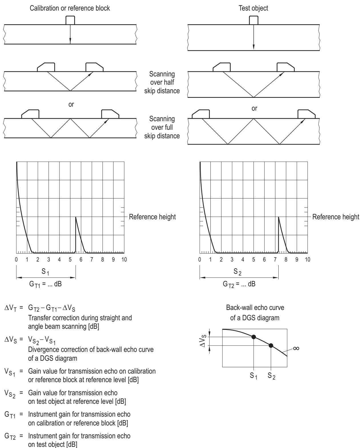
Figure C-5: Determination of transfer correction during straight and angle beam scanning performed as V or W-transmission
