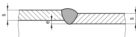
Figure 5-1: Misalignment of welds for vessels and piping
