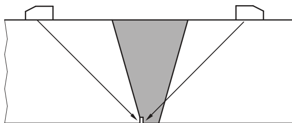
Figure 4-1: Location of notches and beam angles for the test of welded joints between ferritic steels and between austenitic steels
