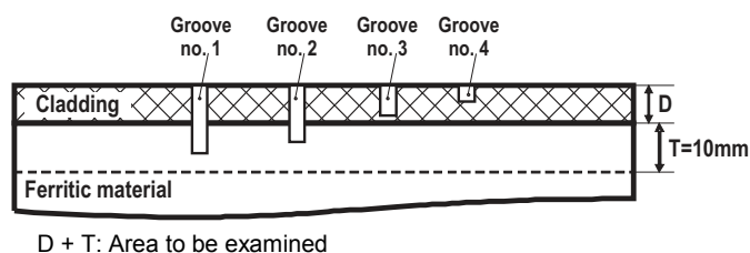
Figure 4-4: Location of notches for the examination of clad surfaces
