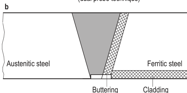
Figure 4-3: Location of notches and beam angles for the examination for transverse defects of welded joints
