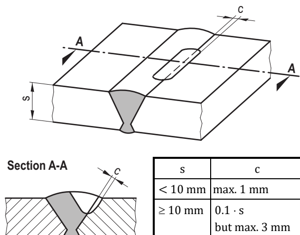
Figure 8-2: Change of the actual weld seam geometry
