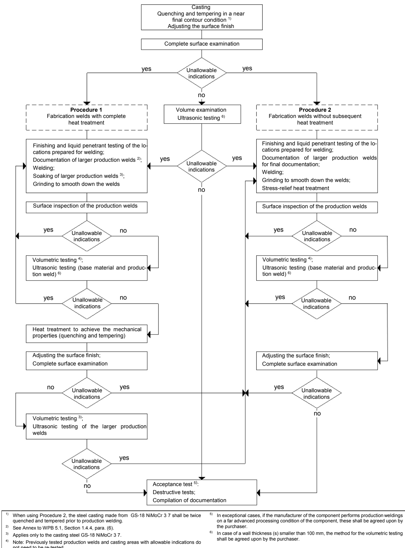
Figure WPB 5.1-1: Standard flow-chart for the production welds on cast steel products
