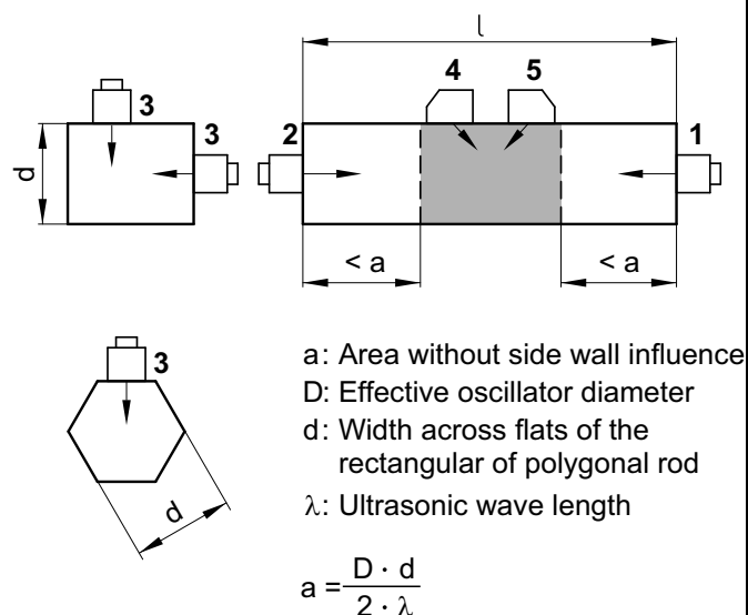
Figure B-2: Scanning positions for rectangular or polygonal bars
