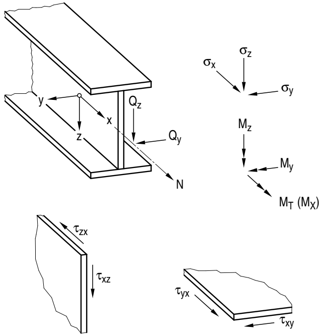
Figure E 2-1: Coordinate system for stress resultants and loadings
