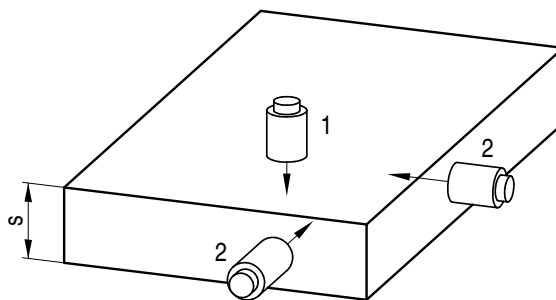
Figure B-3: Scanning positions for plates and sheets
