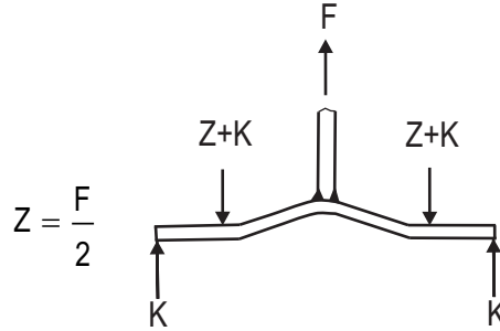
Figure E 4-2: T-joint (based on historic standard DIN 18800-1)
