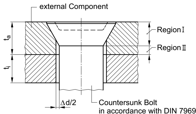
Figure E 4-1: Countersunk head bolted connection in accordance with DIN 7969
