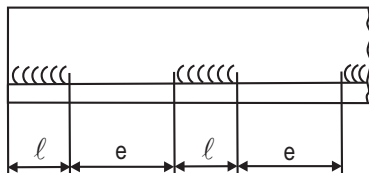
Figure E 3-4: For the analysis of weld seam shear stresses, \tau_{II} , in intermittent welds
