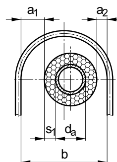
Figure D-2: Loading of the pipe-whip restraint
