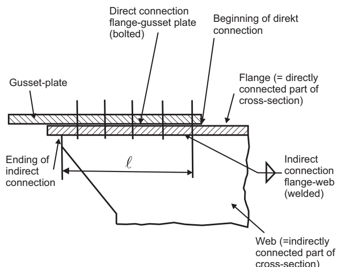
Figure E 3-3: Indirect connection in the case of composite cross-sections (based on historic standard DIN 18800-1)
