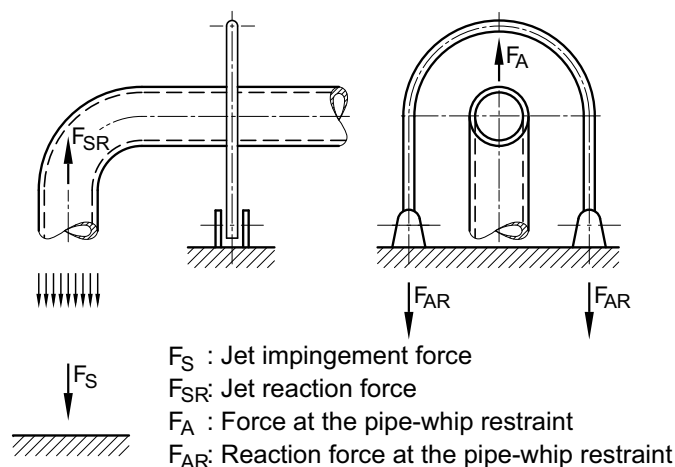
Figure D-1: Notation of forces caused by leaking fluid due to cracking
