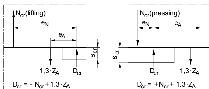
Figure E 5-1: Determination of anchor tensile force
