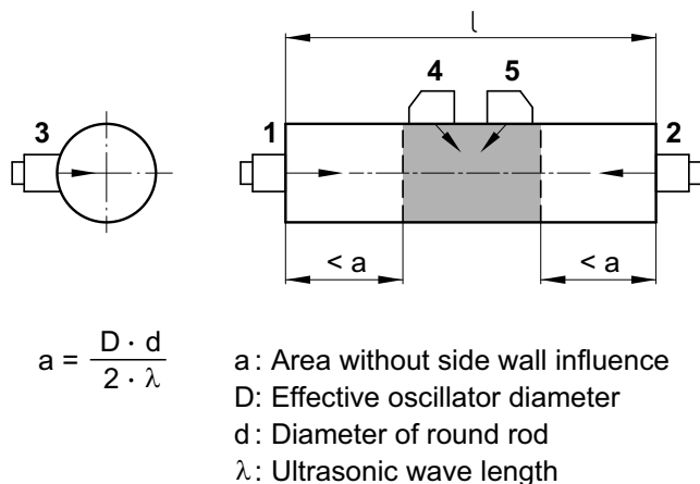
Figure B-1: Scanning positions for round rods
