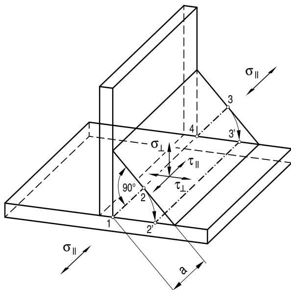
Figure E 3-2: Possible directions of stresses in the fillet weld
