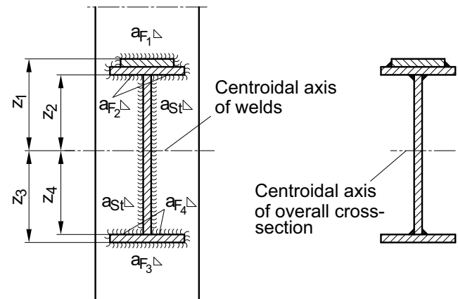
Figure E 3-1: Bending resistant girder (beam) connection
