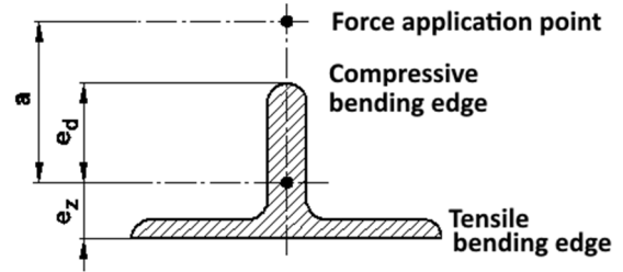
Figure A-2: Bar cross-section with e_z < e_d
