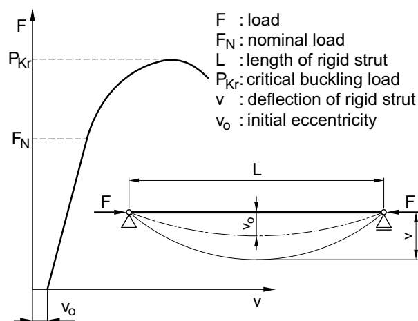
Figure F 4-1: Load-deflection diagram of buckled bars
