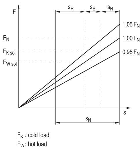
Figure B 2-2: Adjustment range for spring hangers and supports
