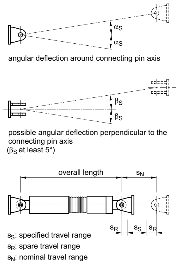
Figure D 2-1: Freedom of movements of a shock absorber
