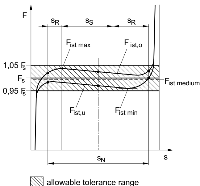
Figure C 2-1: Force-travel diagram for constant hangers and constant supports
