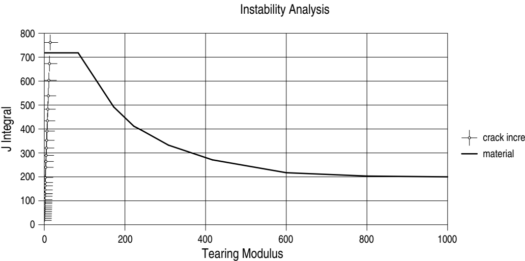
Figure D 2-8: Instability analysis for internal pressure
