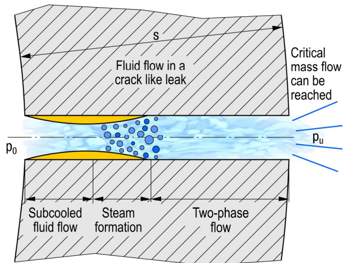
Figure B 3.2-1: Schematic illustration of two-phase discharge flow through a crack
