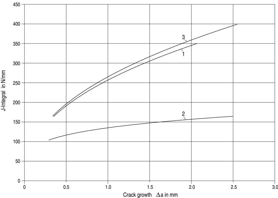
Figure C 2-16: Technical J-R curves for the steel 15NiCuMoNb5
