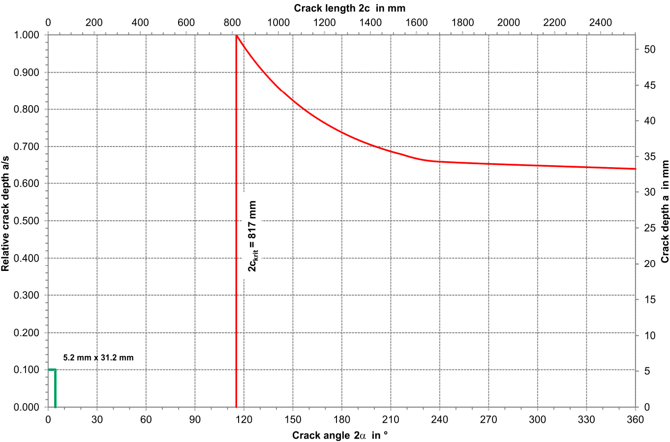
Bild D 2-2: Leak-before-break diagram – plastic limit load approach (PLL)
