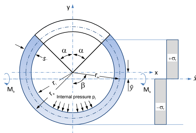
Figure B 2.1-1: PLL – through-thickness crack in circumferential direction
