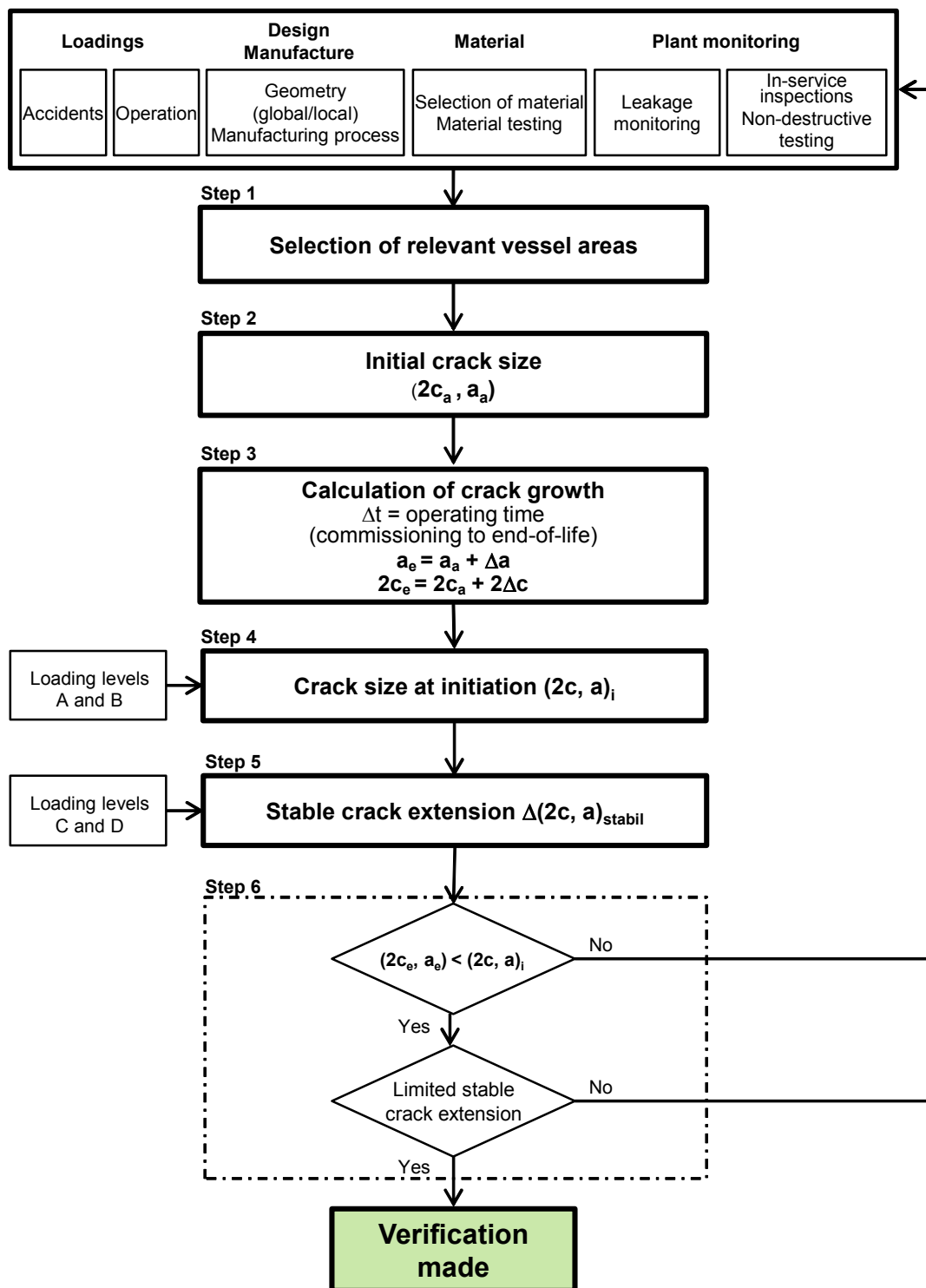
Figure A-5: Fracture mechanics analysis of postulated cracks in pressure vessels
