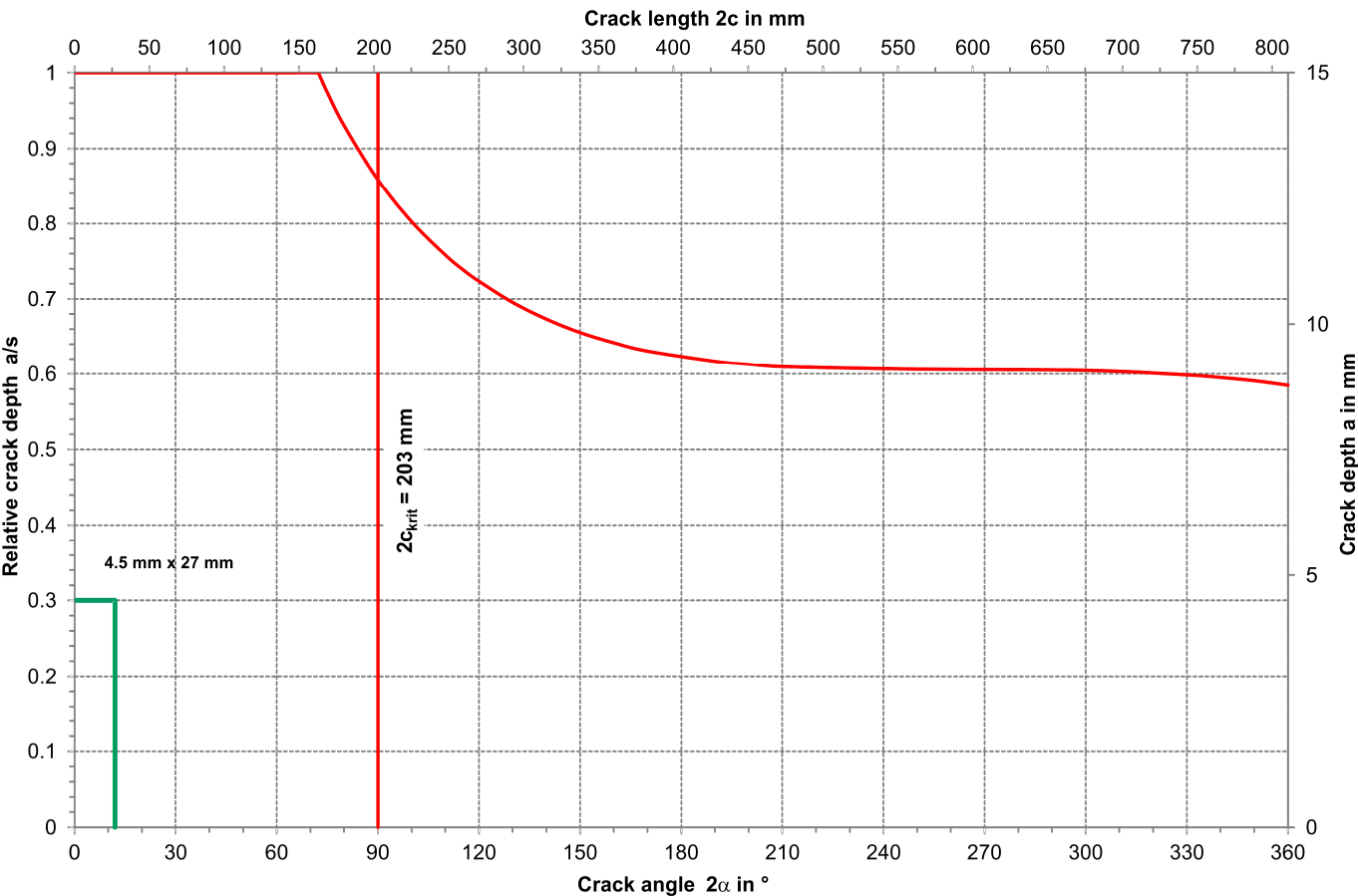
Figure D 1-3: Leak-before-break diagram – FSC / MPA
