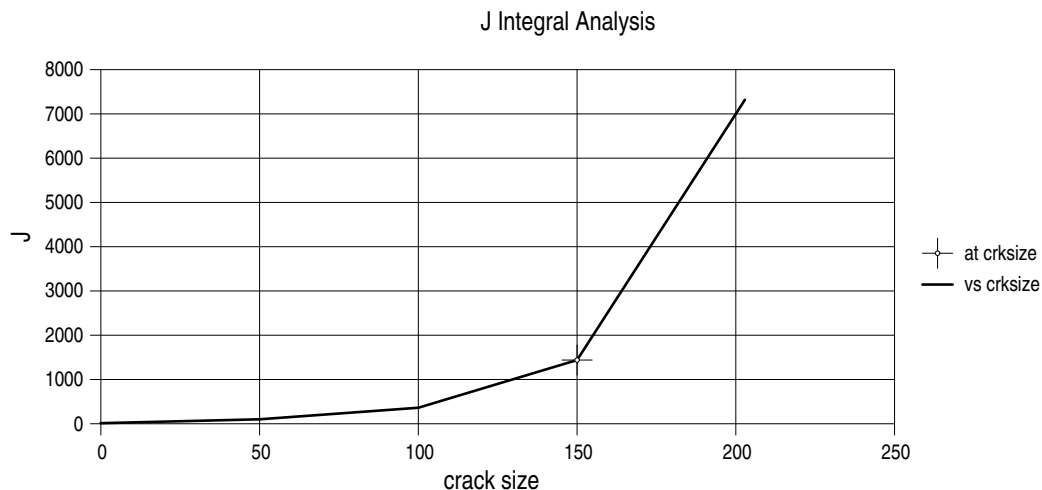
Figure D 1-5: J-integral analysis for bending
