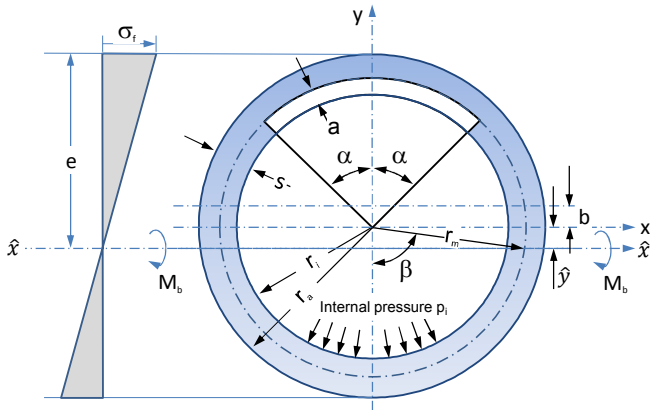
Figure B 2.1-4: FSC/MPA – Surface crack in circumferential direction
