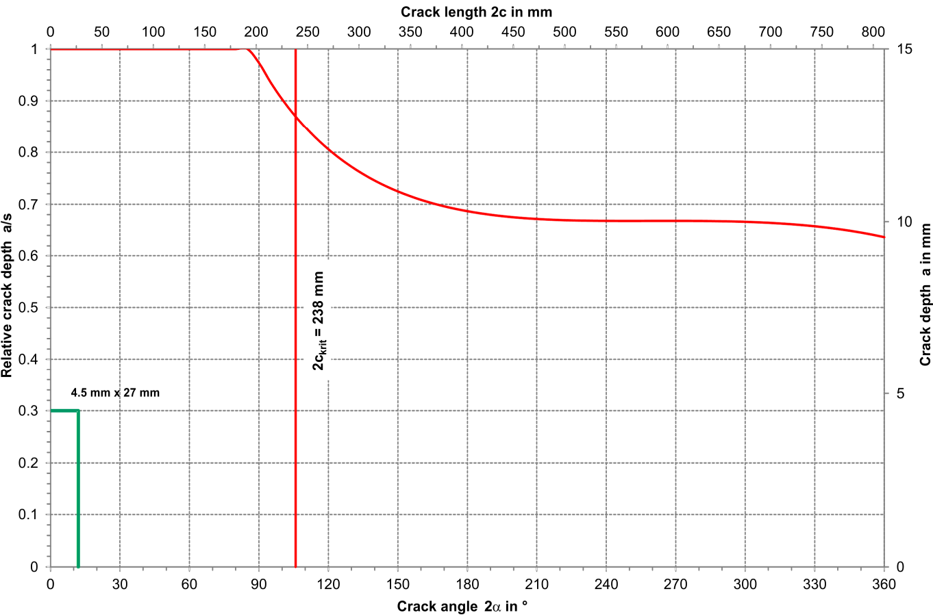
Figure D 1-4: Leak-before-break diagram – FSC / KWU
