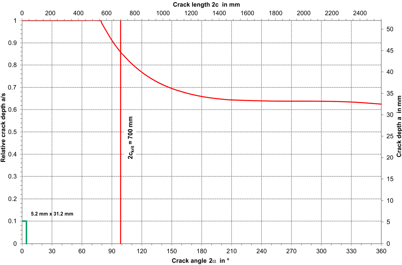
Bild D 2-3: Leak-before-break diagram – FSC / MPA
