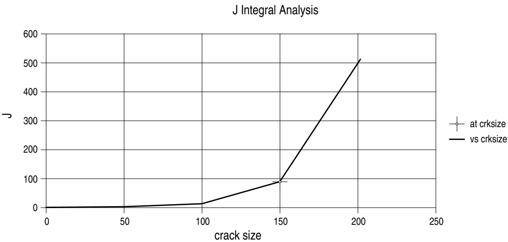
Figure D 1-7: J-integral analysis for internal pressure
