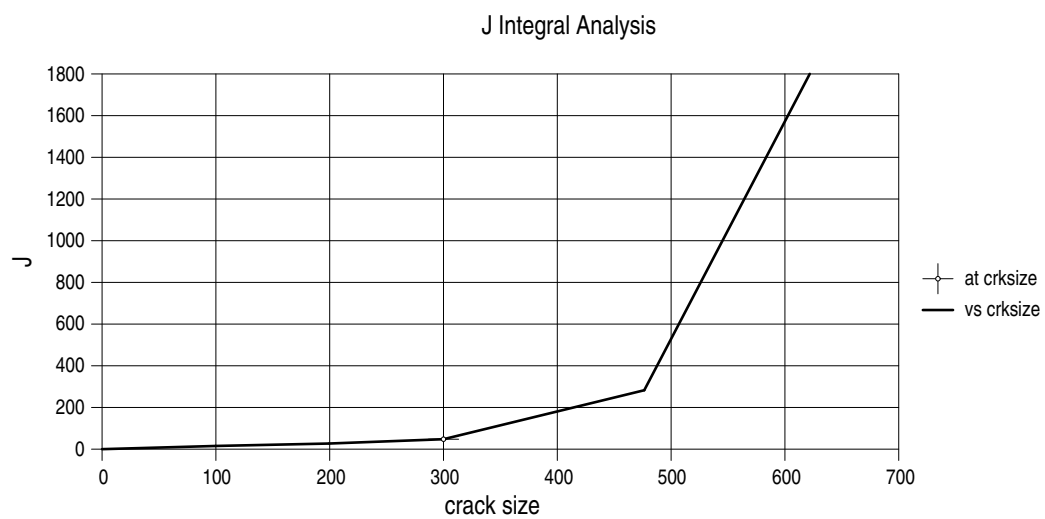
Figure D 2-7: J-integral analysis for internal pressure
