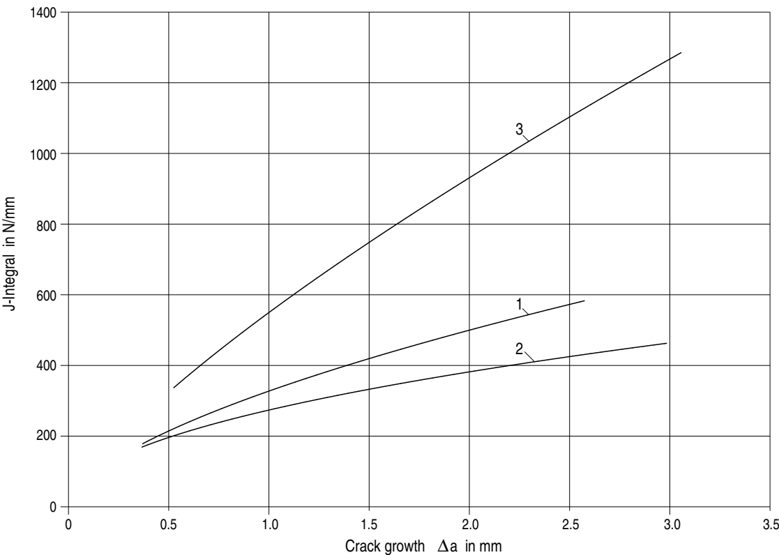
Figure C 2-17: Technical J-R curves for the steel 22NiMoCr3-7
