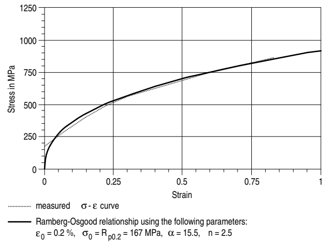
Figure B 2.2-5: True stress-strain curve (schematic)
