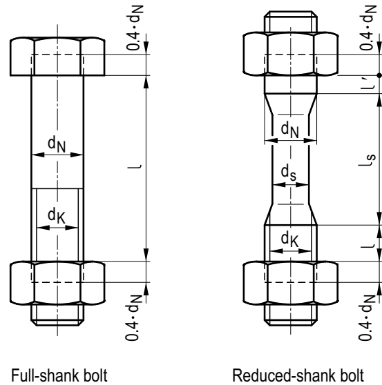
Figure A 2.10-7: Bolts
