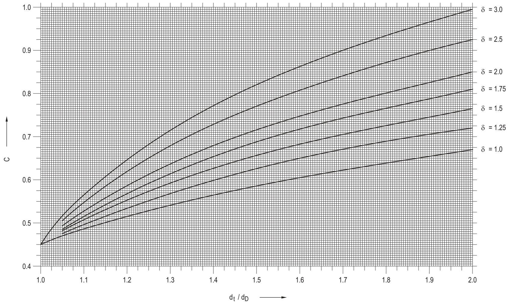
Figure A 2.7-3: Factor C of flat circular plates with additional edge moment acting in same direction (acc. to equation A 2.7-13)
