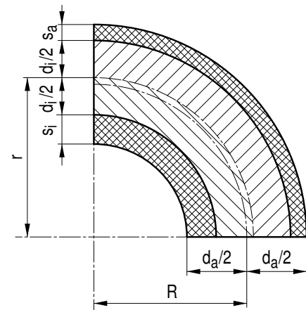
Figure A 5-2: Notations used for pipe bend
