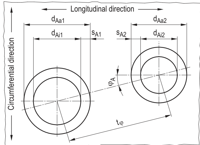
Figure A 5-16: Adjacent openings with differing branch diameters (shown as developed length)
