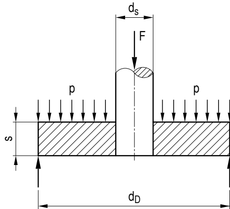
Figure A 2.7-15: Valve disk in the form of a circular ring plate
