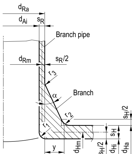
Figure A 5-13: Branch
