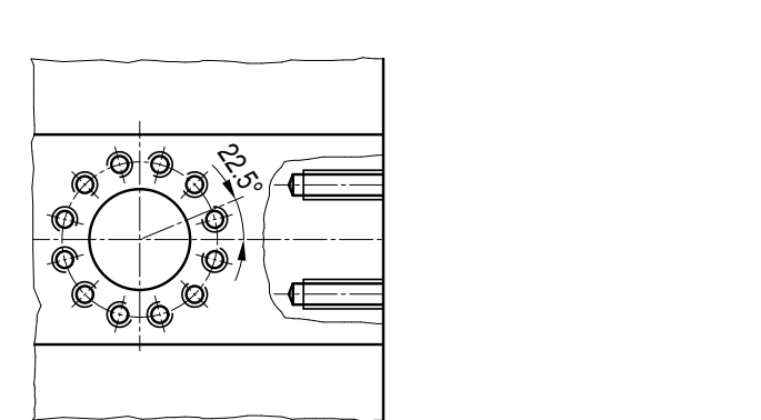
Figure A 3.3-6: Design sketch for consideration of boreholes
