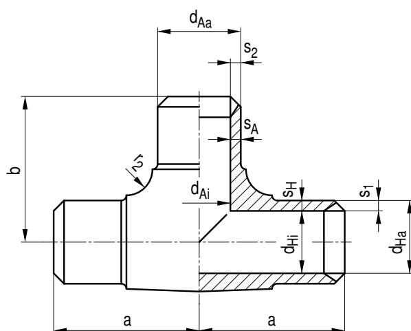
Figure A 5-7: Branch forged from solid, bored or turned
