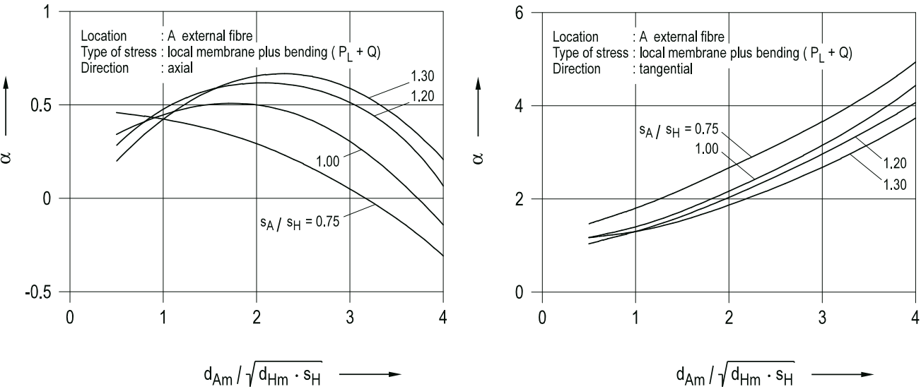
Figure 8.2-8: Stress index \alpha for nozzle in cylindrical shell subject to internal pressure
