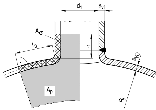
Figure A 2.5-8: Dished head with flanged-out opening
