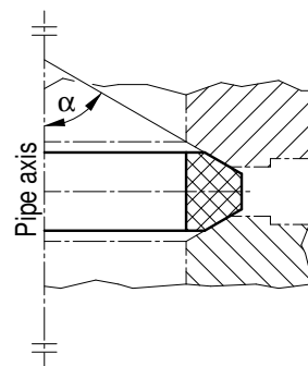
Figure A 2.11-4: Angle \alpha shown with the example of a lens gasket
