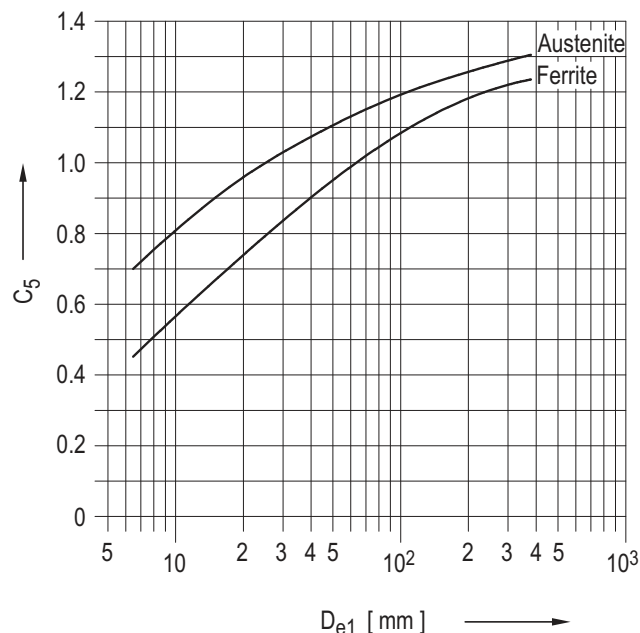
Figure 8.4-12: Stress index C_5 for consideration of thermal fatigue stresses resulting from through-wall temperature gradients caused by step change in fluid temperature
