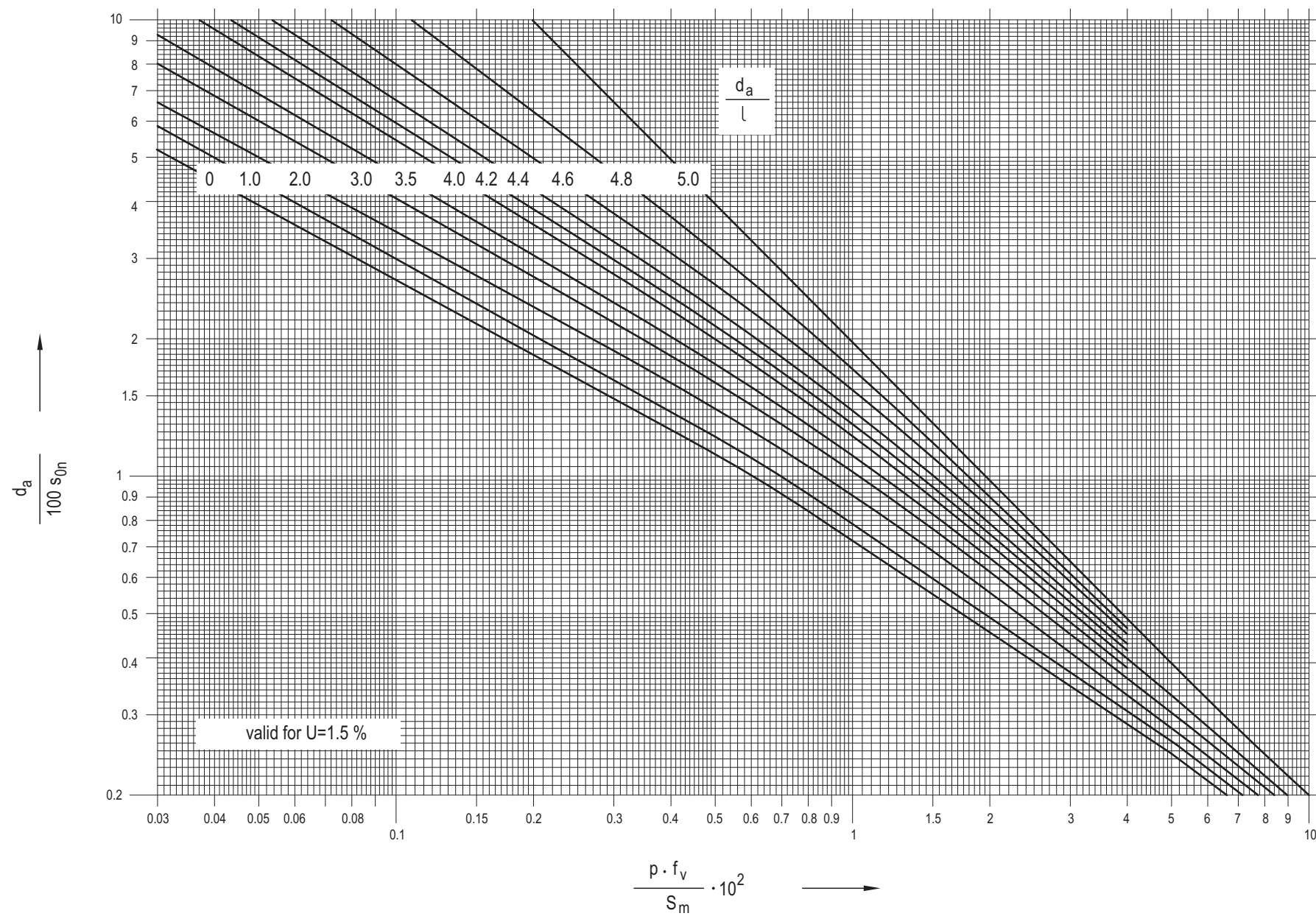
Figure A 2.2-2: Required wall thickness s_{0n} for calculation against gross plastic deformation
