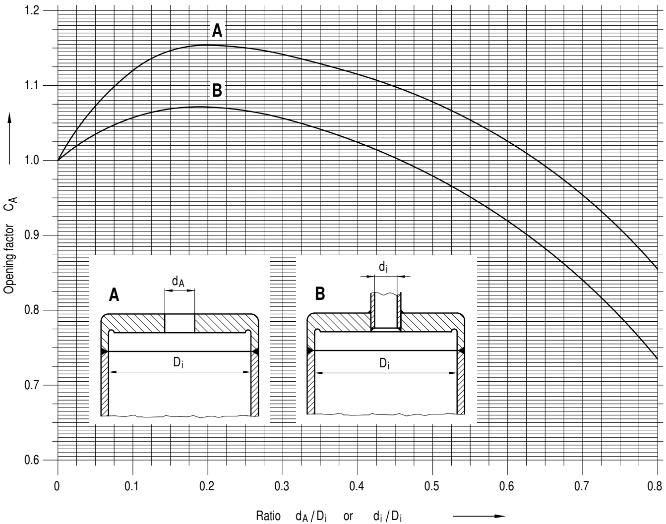
Figure A 3.3-7: Opening factor C_A
