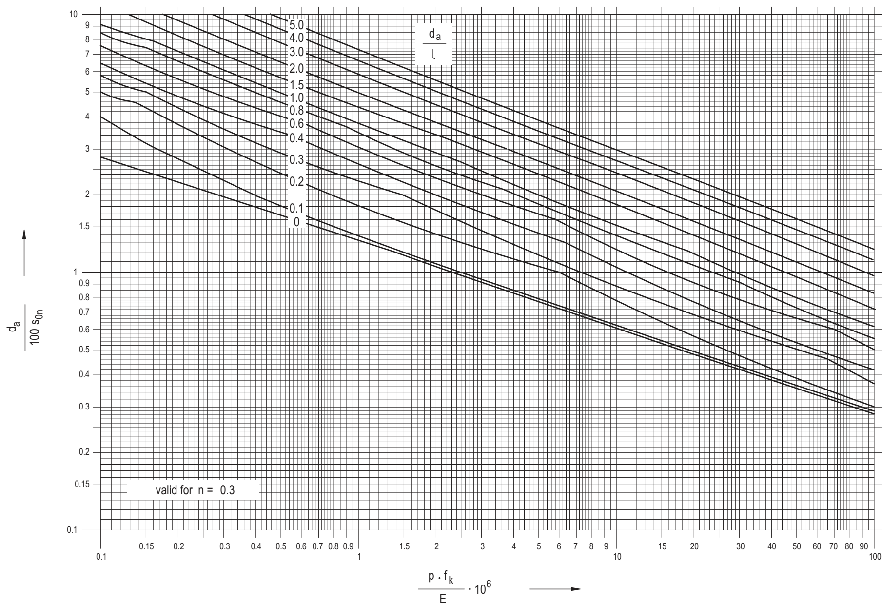
Figure A 2.2-1: Required wall thickness s_{0n} for calculation against elastic instability
