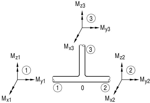
Figure 8.5-6: Designation of moments on branch connection
