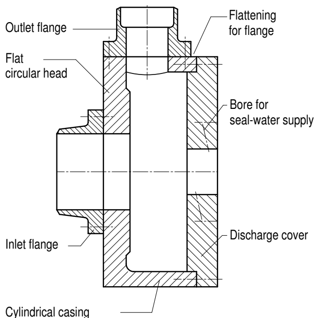
Figure A 3.2-1: Example of a single-stage annular casing pump with forged casing
