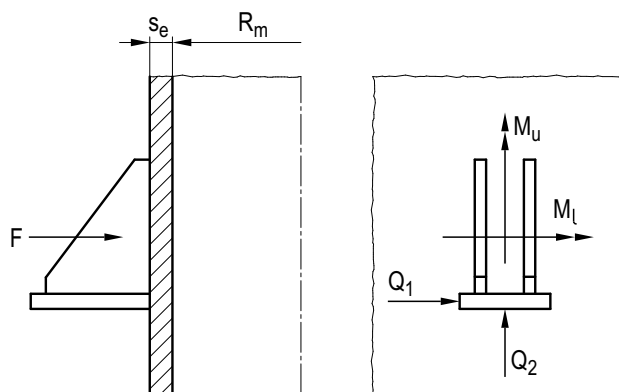
Figure 8.2-19: Vessels with support brackets
