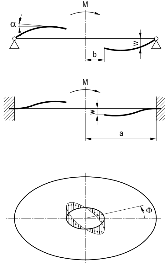
Figure 8.3-1: Course of edge force due to bending moment M ; Design values
