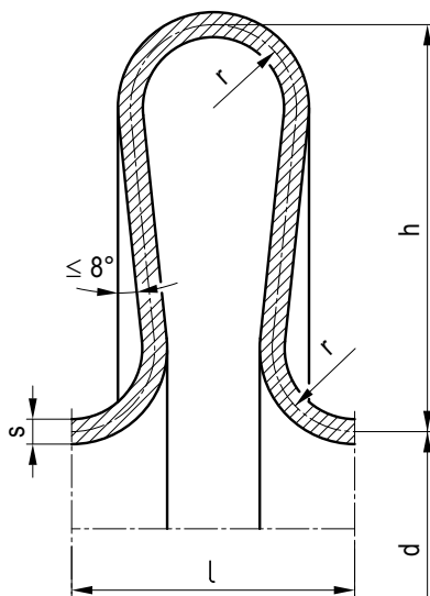
Figure 8.2-13: Slightly lyra-shaped convolution of bellows expansion joint (angle \leq 8^\circ )
