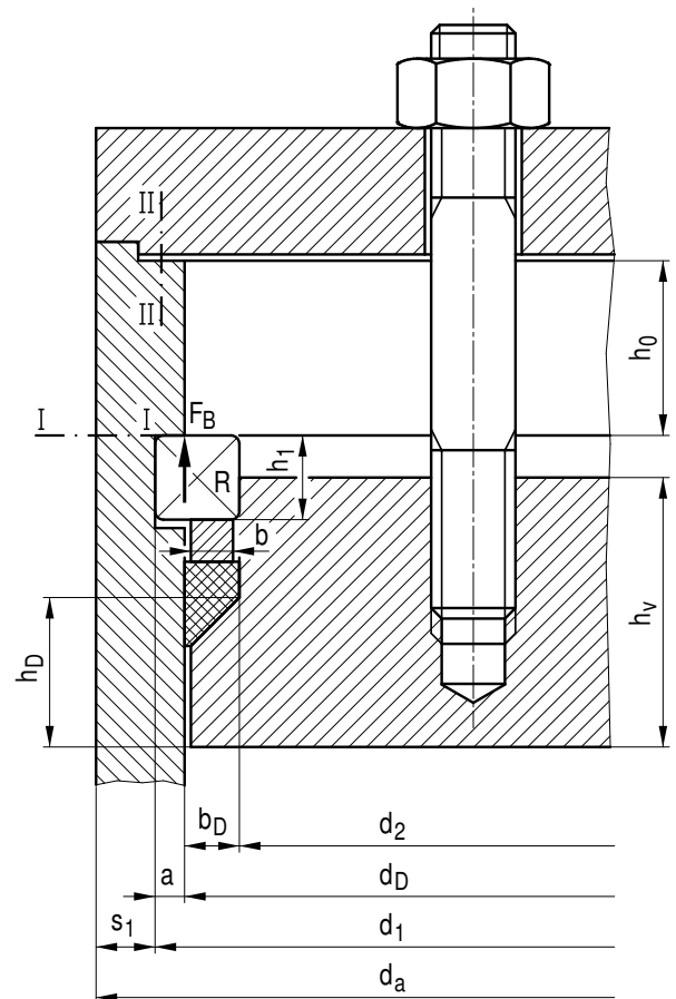
Figure A 4.4-1: Self-sealing cover plates
