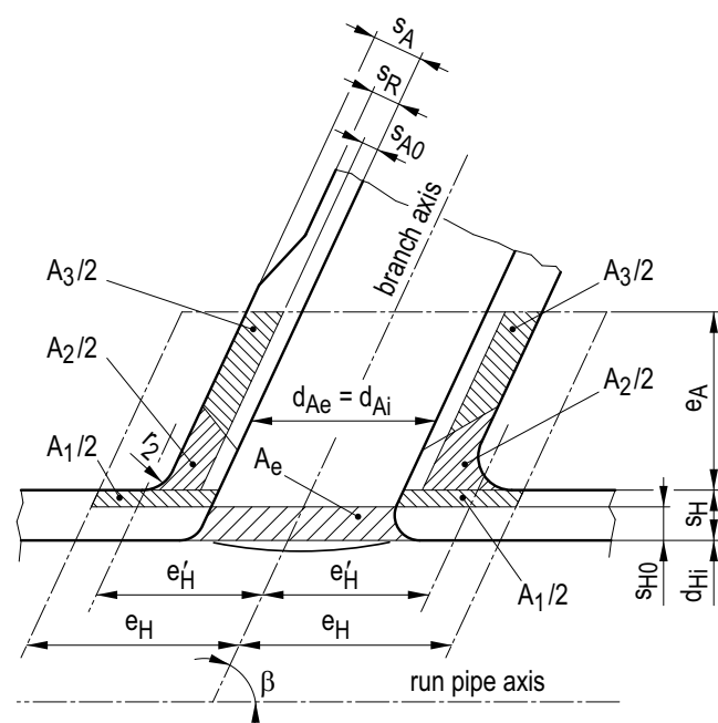
Figure A 2.8-8: Oblique cylindrical branch
