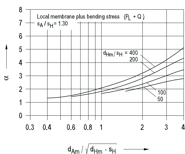
Figure 8.2-11: Stress index \alpha for nozzle in spherical shell subject to internal pressure for P_L + Q
