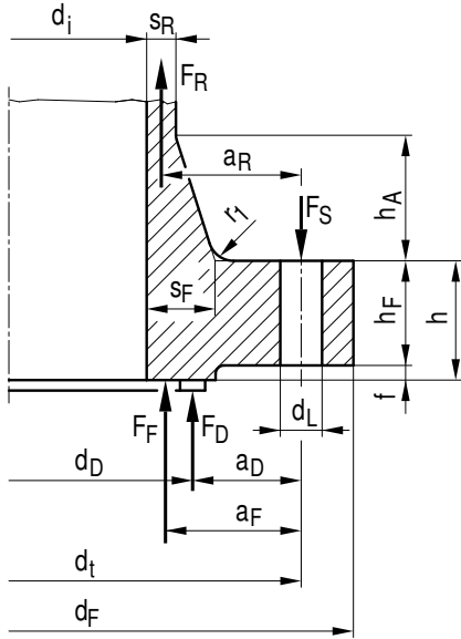
Figure A 2.10-2: Welding-neck flange with tapered hub
