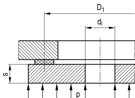
Figure A 2.7-5: Inside circular plate with opening
