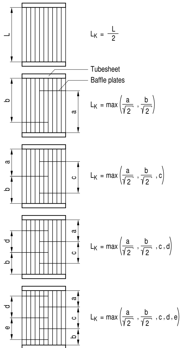
Figure 8.2-18: Determination of buckling length L_K
