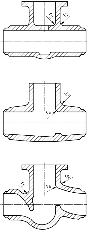
Figure 8.4-2: Fillets and corners
