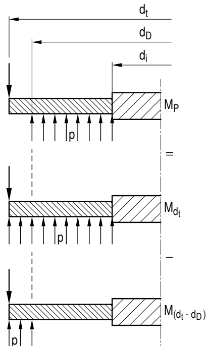
Figure A 2.7-10: Superposition for internal pressure
