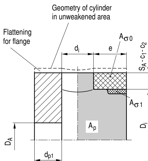
Figure A 3.3-3: Design sketch for annular casings with flattening and opening
