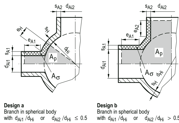
Figure A 4.1-11: Spherical bodies
