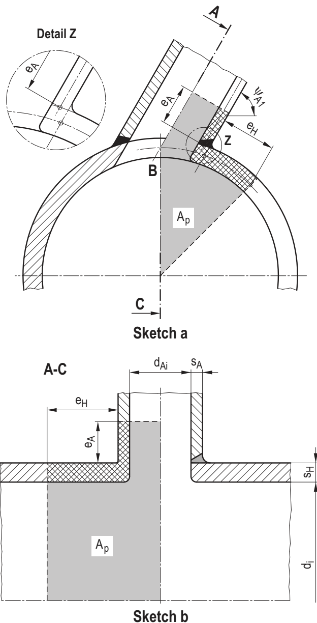
Figure A 5-18: Loading scheme for a cylindrical shell with non-radial branch
