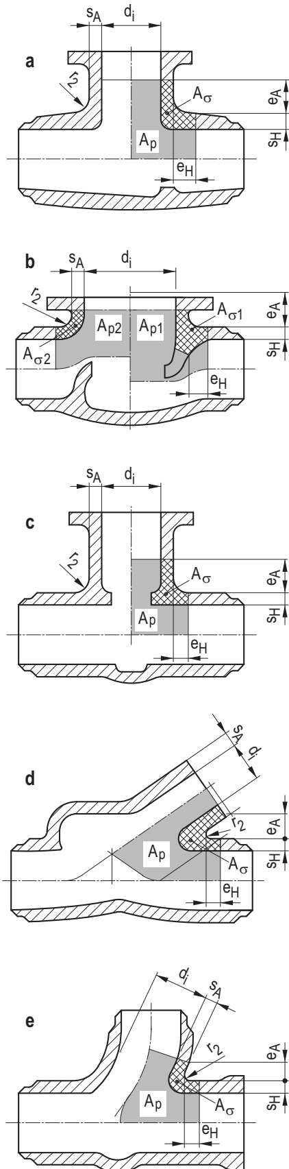
Figure 8.4-1: Pressure area method
