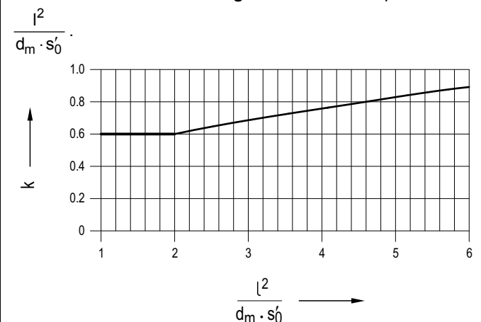
Figure A 4.1-4: Correction factor k for short bodies
