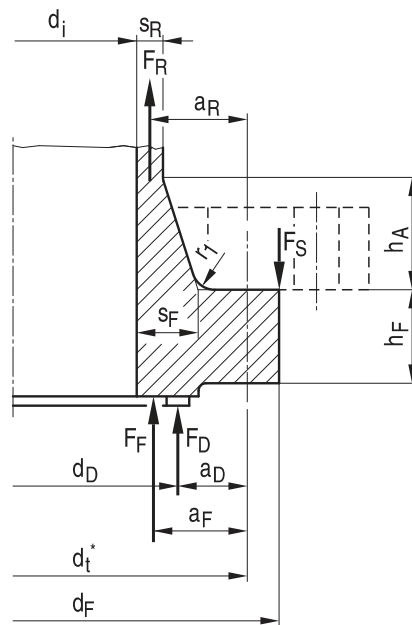
Figure A 2.10-3: Welding stub with tapered hub
