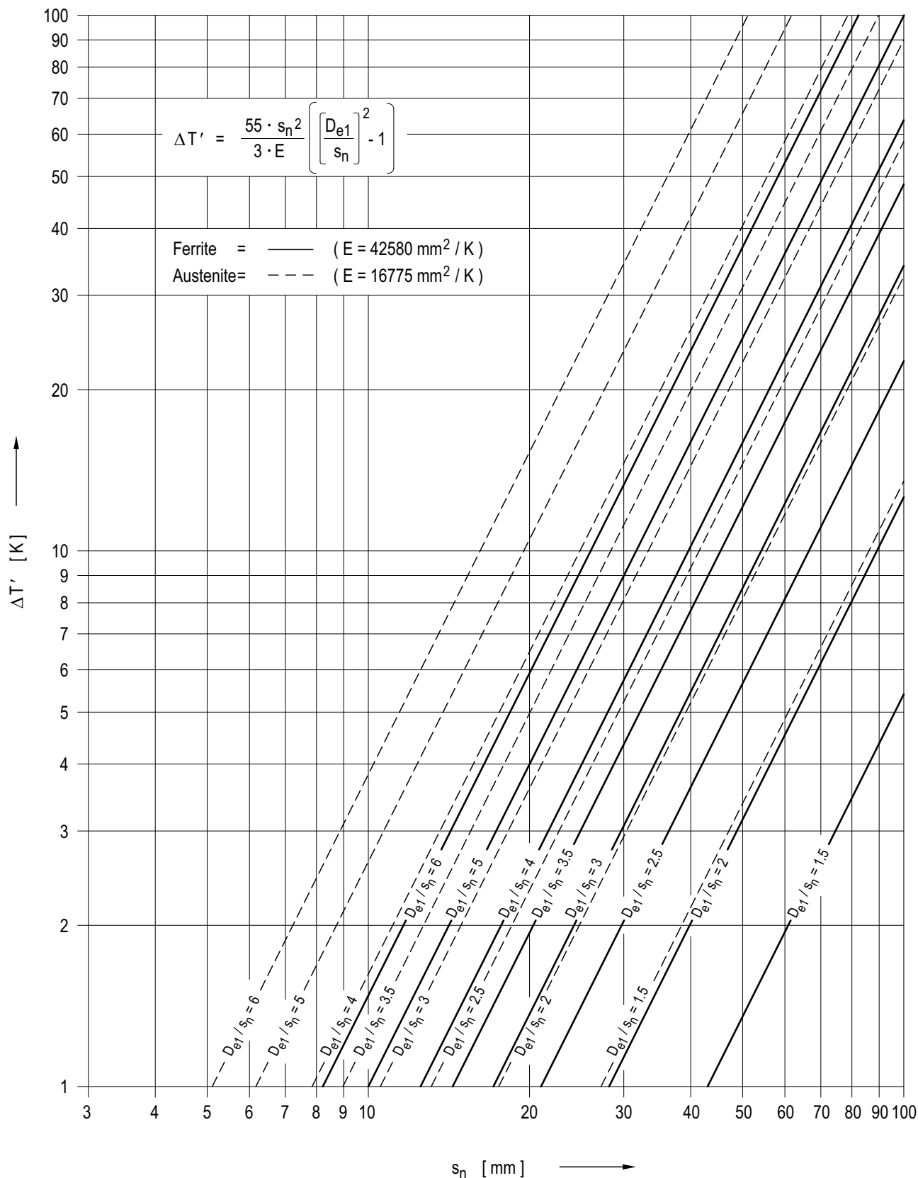
Figure 8.4-9: Maximum temperature difference in valve body (area D_{e1}/s_n ), associated with a fluid temperature change rate of 55 K/hr
