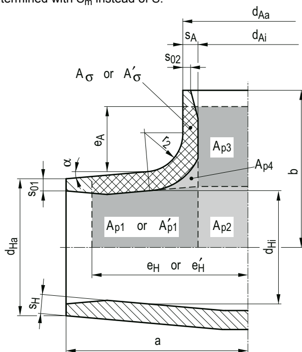
Figure A 5-9: Reinforcement area dimensions for butt welding tees
