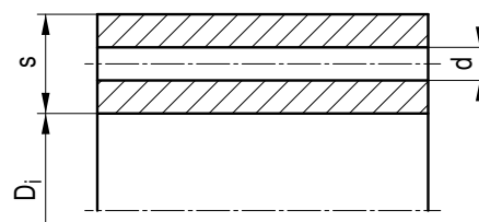
Figure A 3.4-2: Borehole in cylindrical shell
