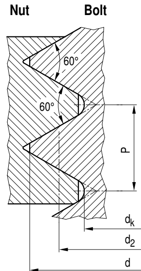
Figure A 2.9-8: Thread dimensions
