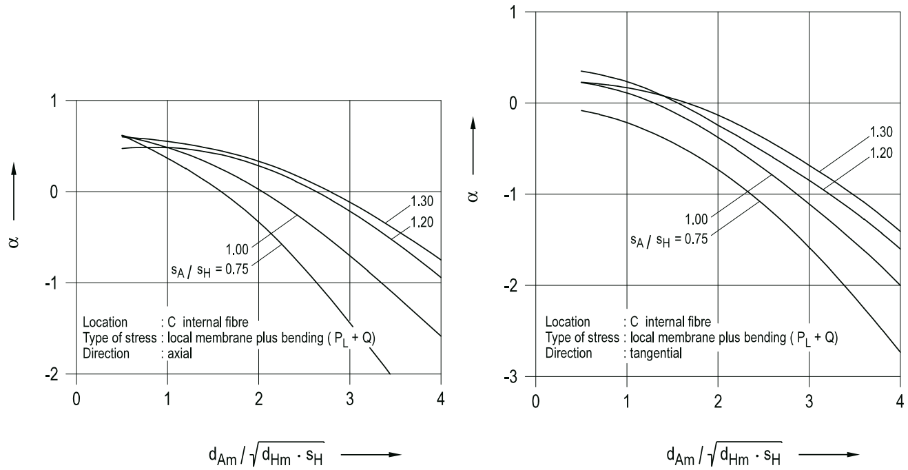
Figure 8.2-7: Stress index \alpha for nozzle in cylindrical shell subject to internal pressure
