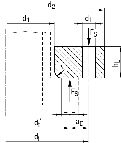
Figure A 2.10-6: Lap-joint flange
