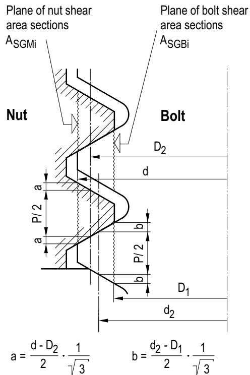
Figure A 2.9-3: Representation of design values for bolt and female thread
