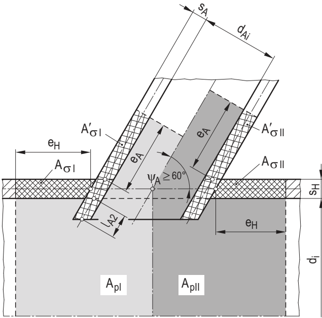
Figure A 5-14: Loading scheme for a cylindrical shell with oblique branch
