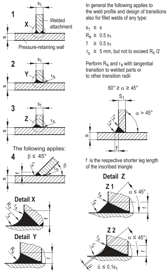
Figure 5.2-2: Examples of single-bevel and double-bevel butt welds for attachment welds
