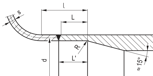
Figure 5.3-2: Example of connection between expansion joint and vessel
