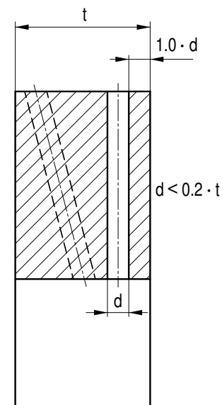
Figure A 3.4-1: Boreholes in casing cover
