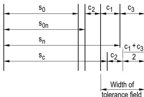
Figure 7.1-1: Wall thicknesses
