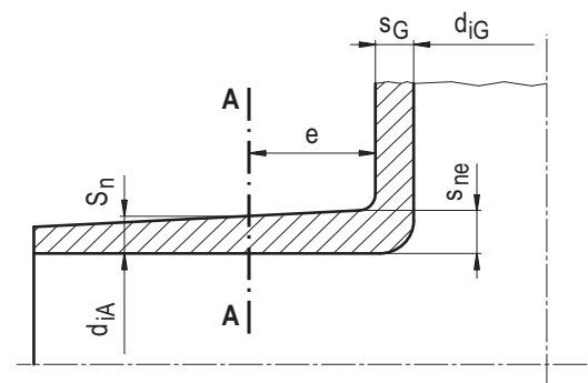
Figure 8.4-4: Critical sections of valve bodies
