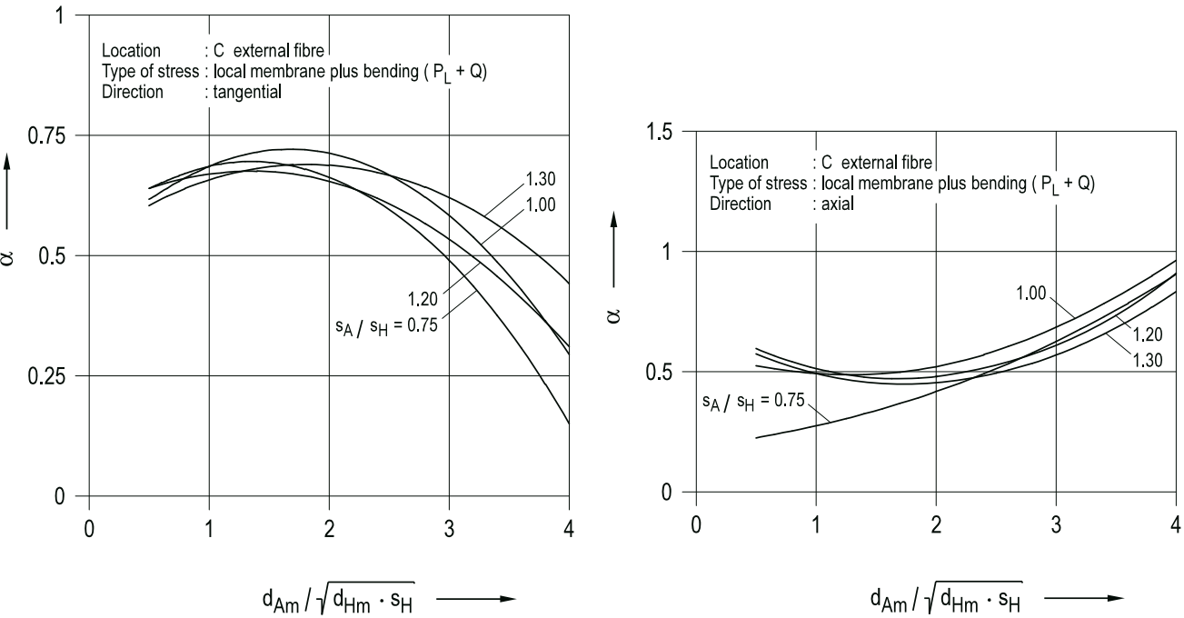
Figure 8.2-9: Stress index \alpha for nozzle in cylindrical shell subject to internal pressure
