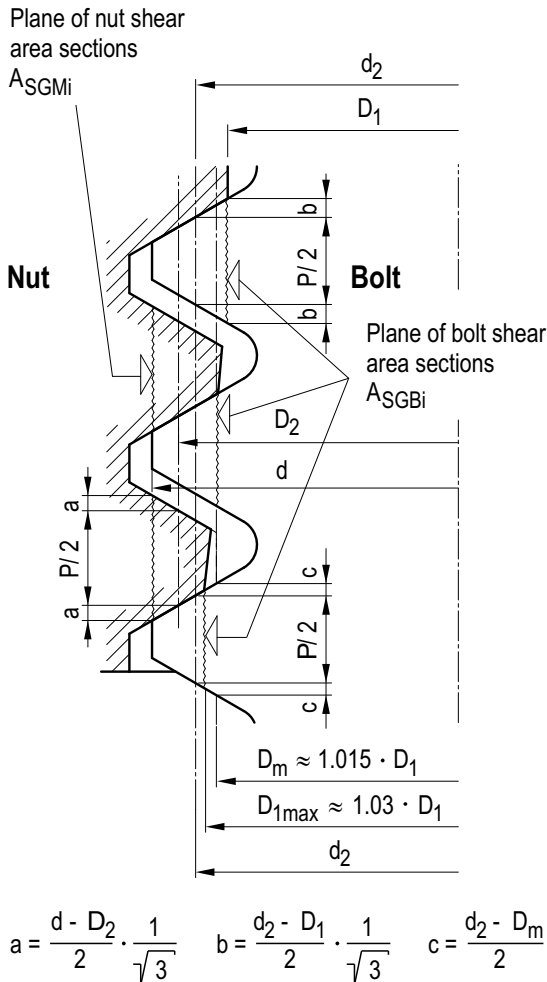
Figure A 2.9-4: Representation of design values for bolt and female thread (tapered female thread)
