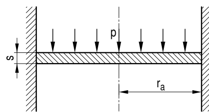
Figure A 2.7-8: Clamped flat head
