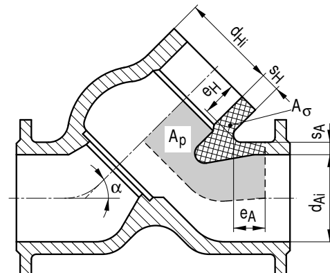
Figure A 4.1-14: Cylindrical body with oblique branch
