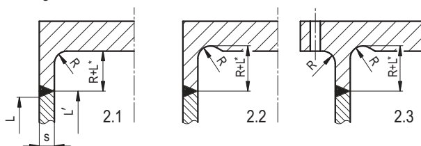
Figure 5.3-2: Example of connection between expansion joint and vessel
