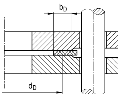
Figure A 2.11-2: Gasket width b_D
