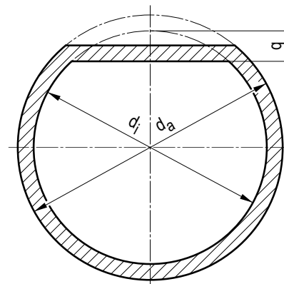
Figure 7.1-2 : Flattening q
