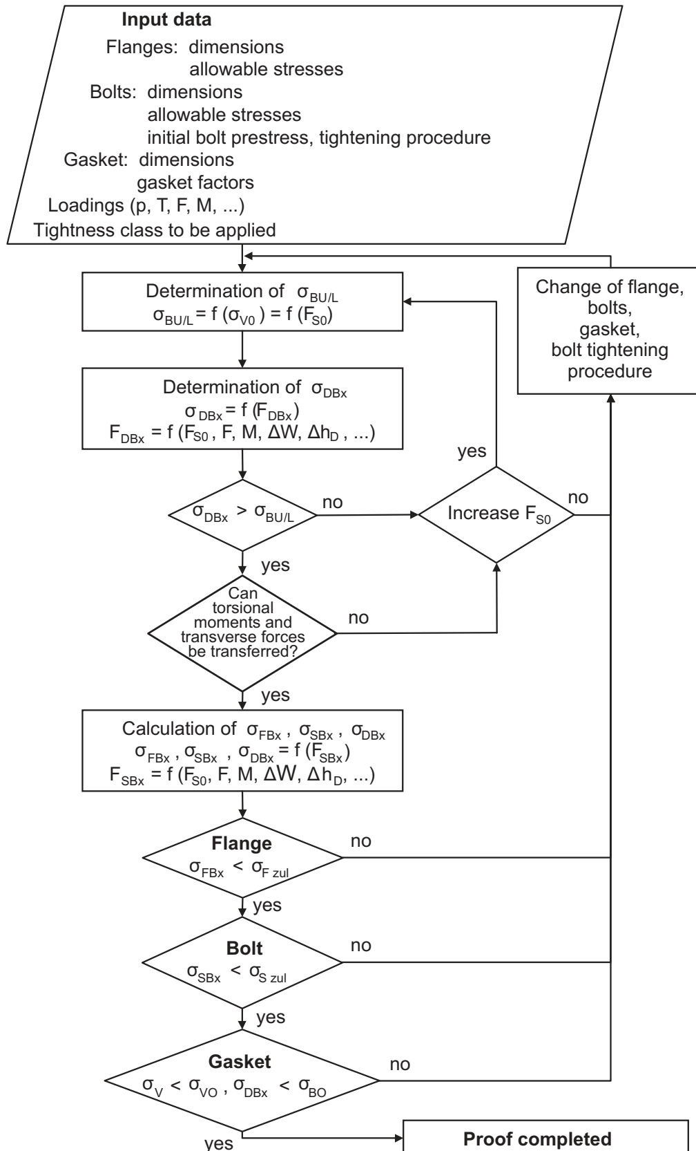
Figure A 2.10-8: Schematic procedural steps for verification of strength of floating type flanged joints
