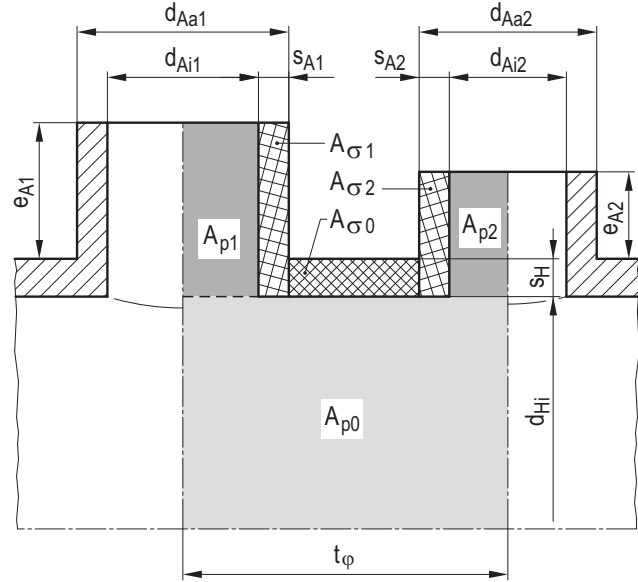
Figure A 5-15: Adjacent openings with differing branch diameters (shown for \varphi_A = 0 )
