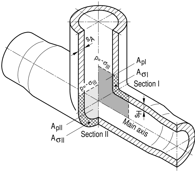
Figure A 4.1-5: Calculated sections for valve bodies with branch
