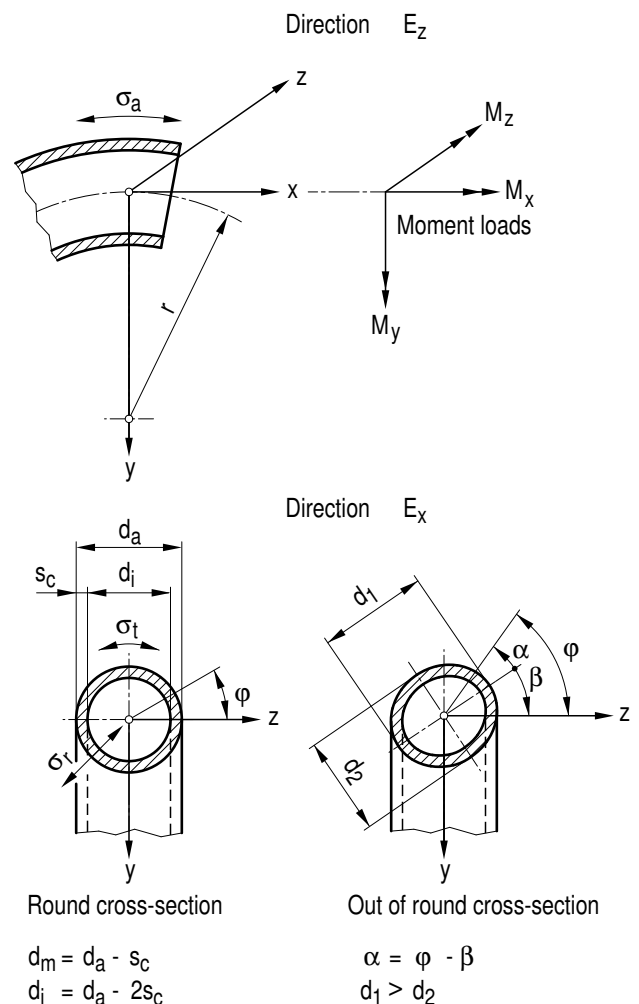
Figure 8.5-8: Pipe elbow nomenclature for detailed stress analysis
