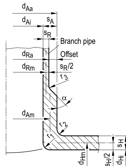
Figure A 5-10: Branch
