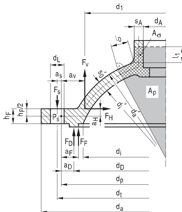
Figure A 2.6-2: Spherically dished head with deep-dished spherical shell (type II, y = 0 )
