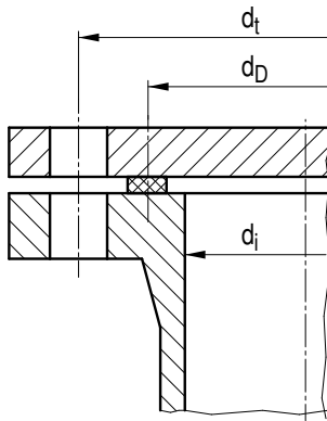
Figure A 2.7-2: Circular flat plate with additional edge moment
