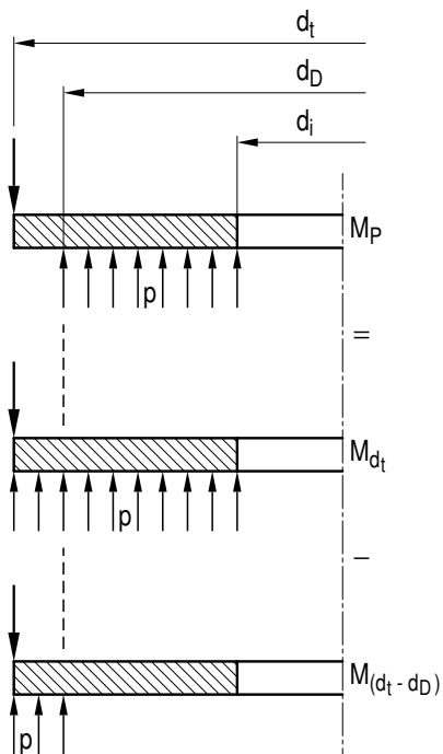
Figure A 2.7-12: Superposition for internal pressure
