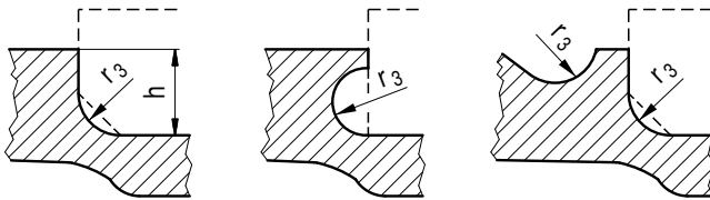
Figure 8.4-3: Acceptable ring grooves
