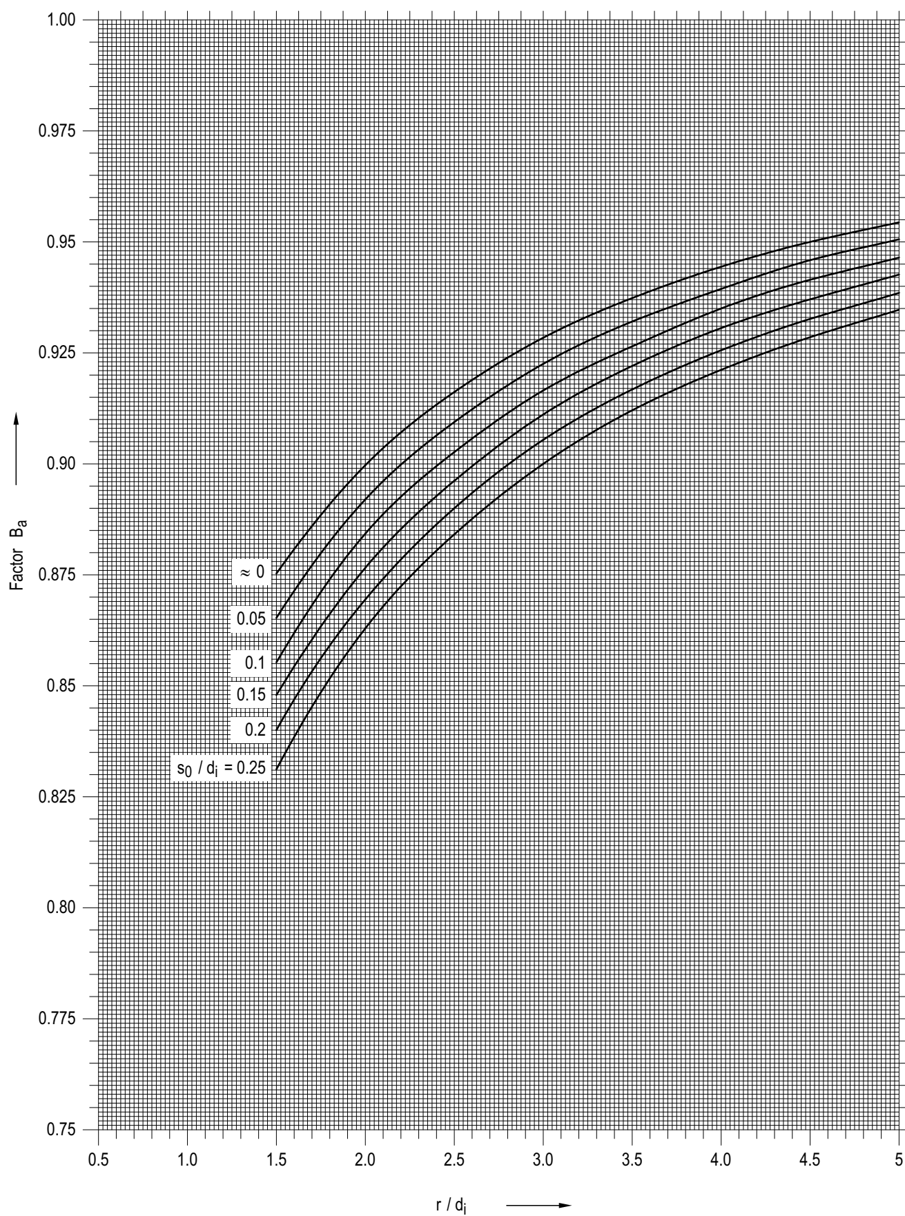
Figure A 5-5: Factor B_a for the extrados at given inside diameter
