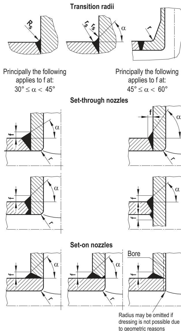
Figure 5.2-4: Designs of welds on nozzles
