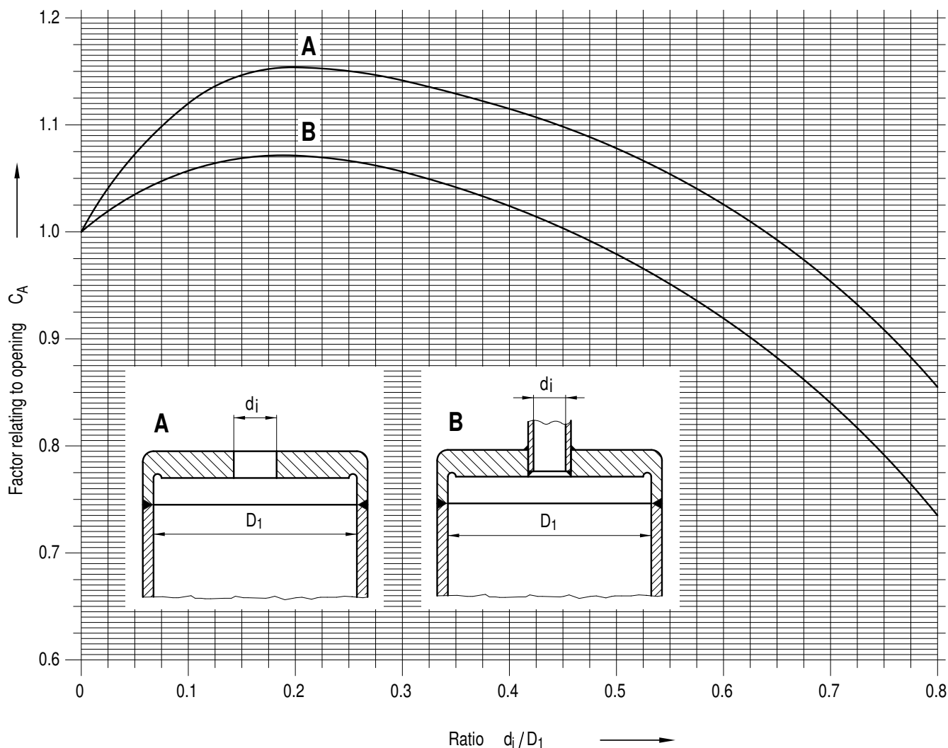
Figure A 2.7-6: Factor C_A relating to opening for stayed circular plate with opening
