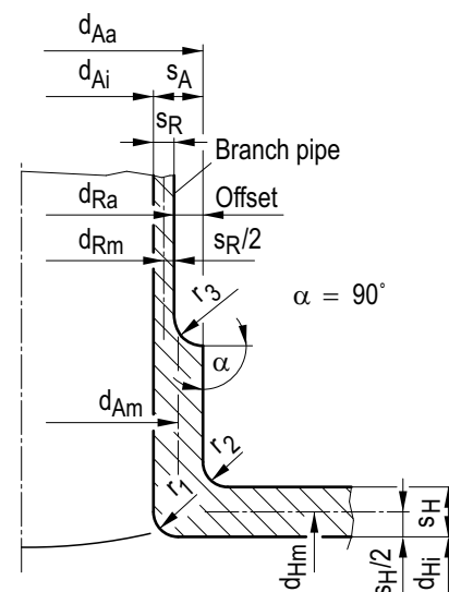
Figure A 5-11: Branch
