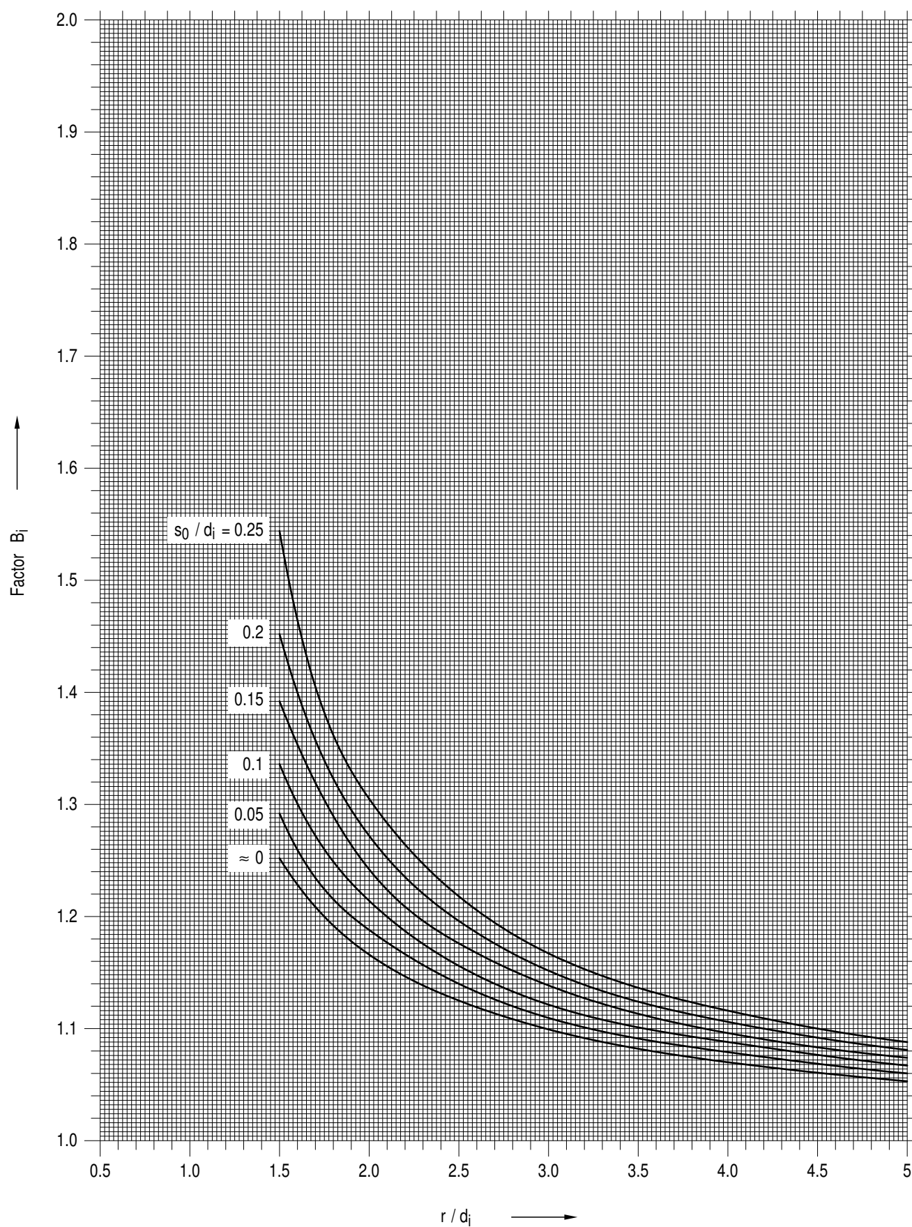
Figure A 5-3: Factor B_i for the intrados at given inside diameter
