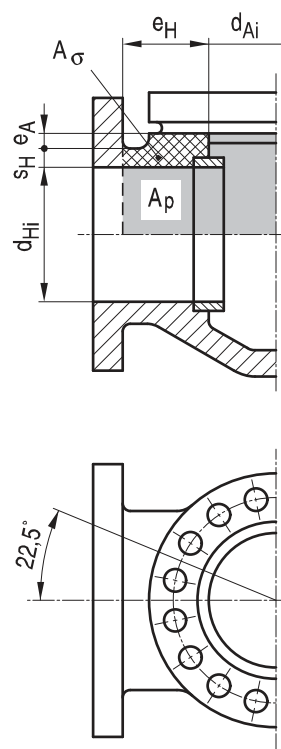
Figure A 4.1-7: Valve body
