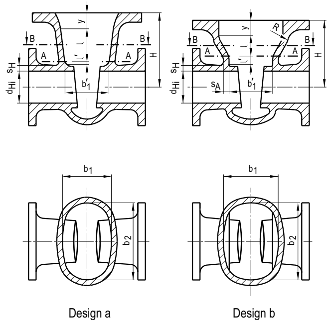
Figure A 4.1-3: Examples for changes in cross-section of oval bodies
