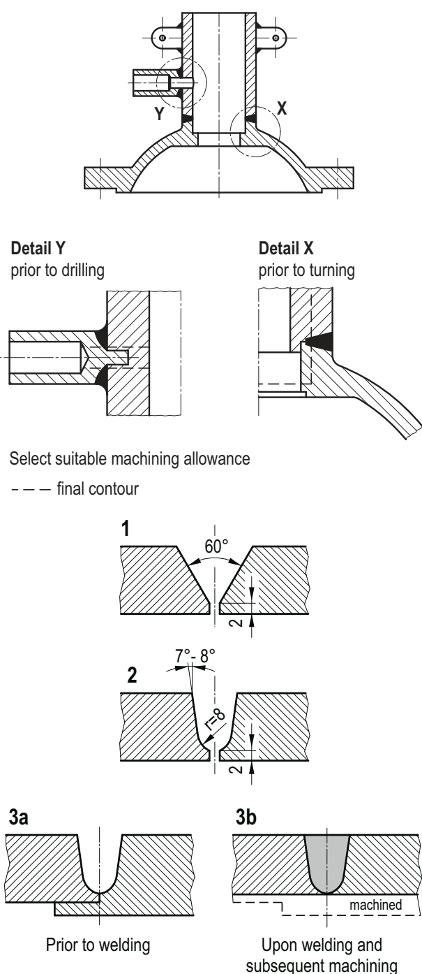
Figure 5.2-1: Examples of single-side butt welds
