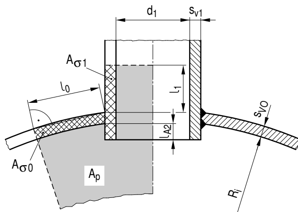
Figure A 2.5-7: Dished head with branch (welded-in tubular reinforcement)
