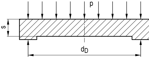
Figure A 2.7-13: Circular flat plate
