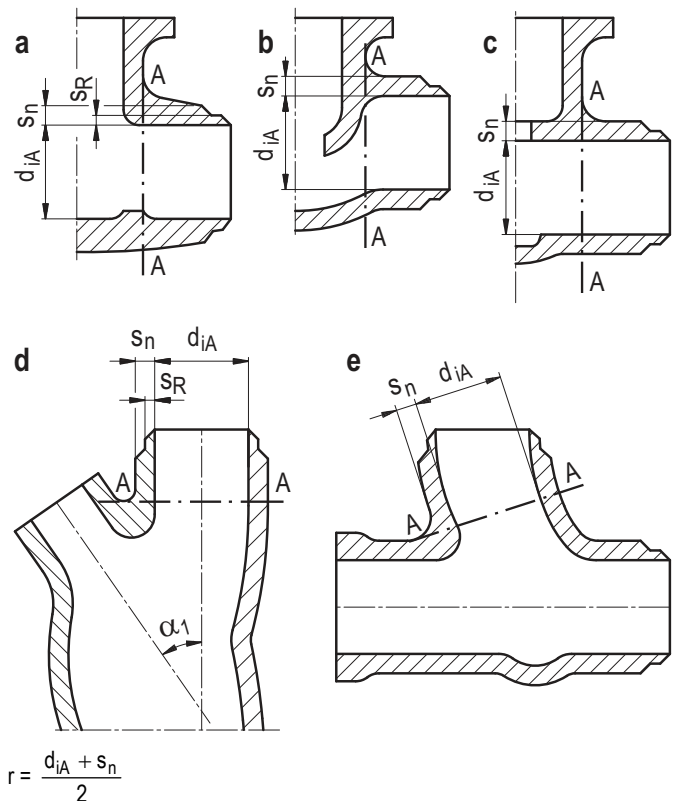
Figure 8.4-4: Critical sections of valve bodies
