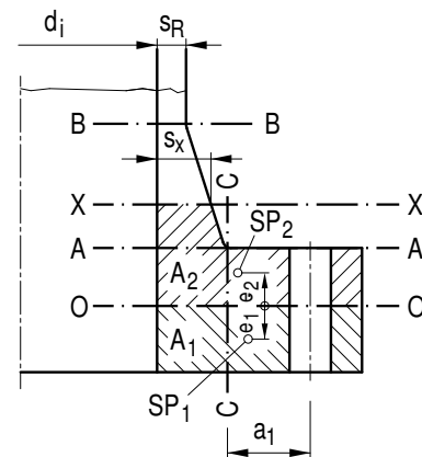
Figure A 2.10-1: Flange cross-section
