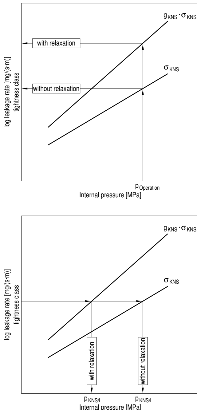
Figure A 2.11-5: Determination of leakage rate (top) and of the sealable pressure (bottom) for metal-to-metal contact type flanged joints (schematically shown)
