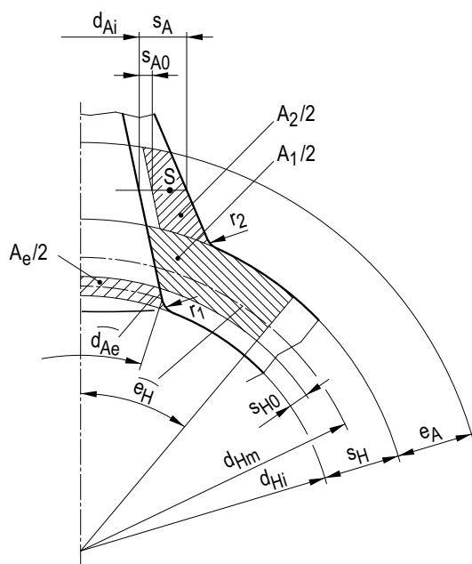
Figure A 2.8-11: Conical branch in spherical shell
