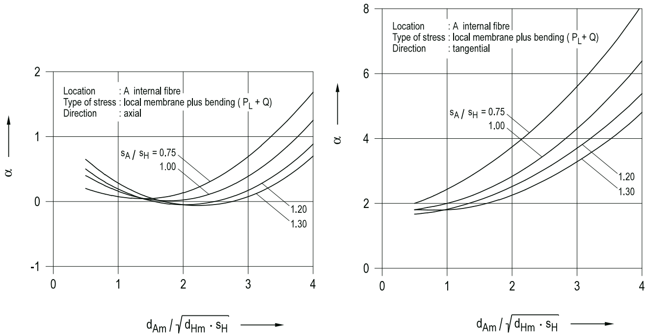
Figure 8.2-6: Stress index \alpha for nozzle in cylindrical shell subject to internal pressure
