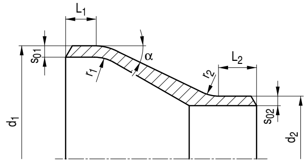
Figure 8.5-5: Concentric reducer
