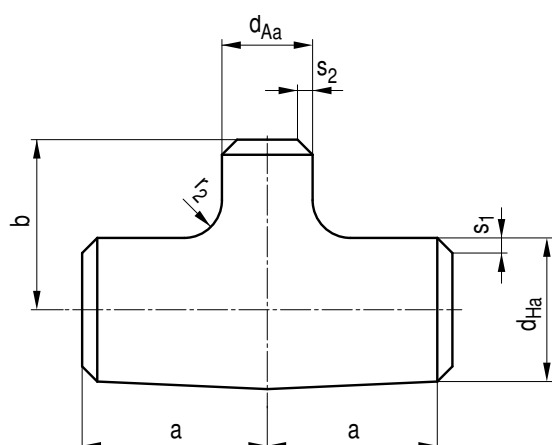
Figure A 5-8: Die-formed butt-welding tee
