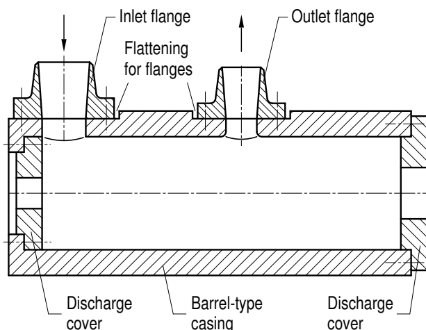
Figure A 3.2-3: Example of a multi-stage barrel-type pump with forged casing
