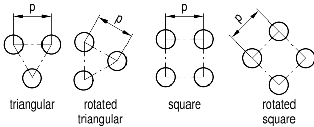
Figure 8.2-16: Tube pattern in tubesheet
