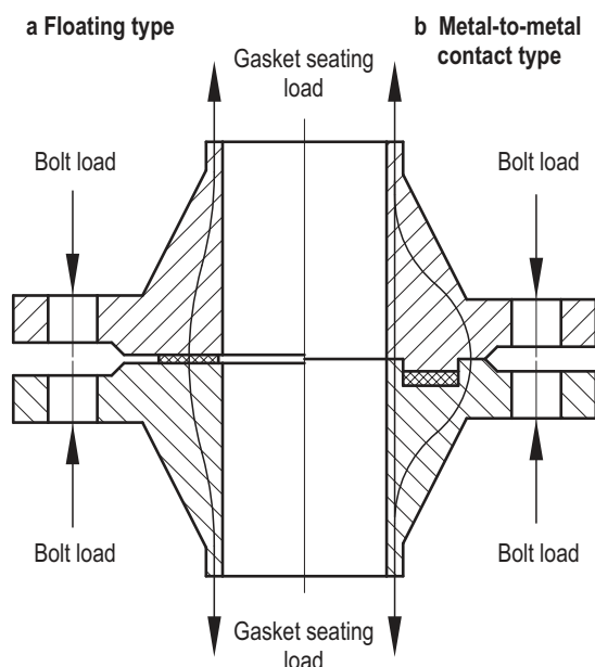
Figure A 2.9-1: Presentation of floating type and metal-to-metal contact type flanged joint (schematic)
