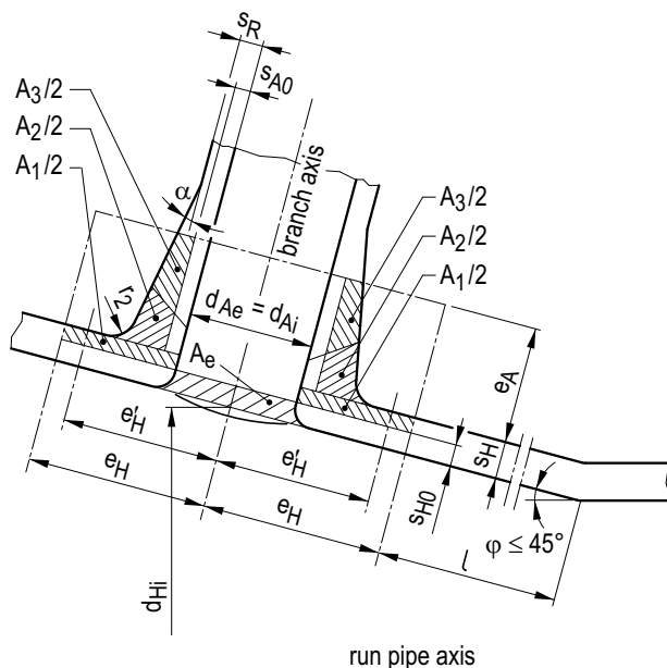
Figure A 2.8-10: Conical shell with reinforced opening
