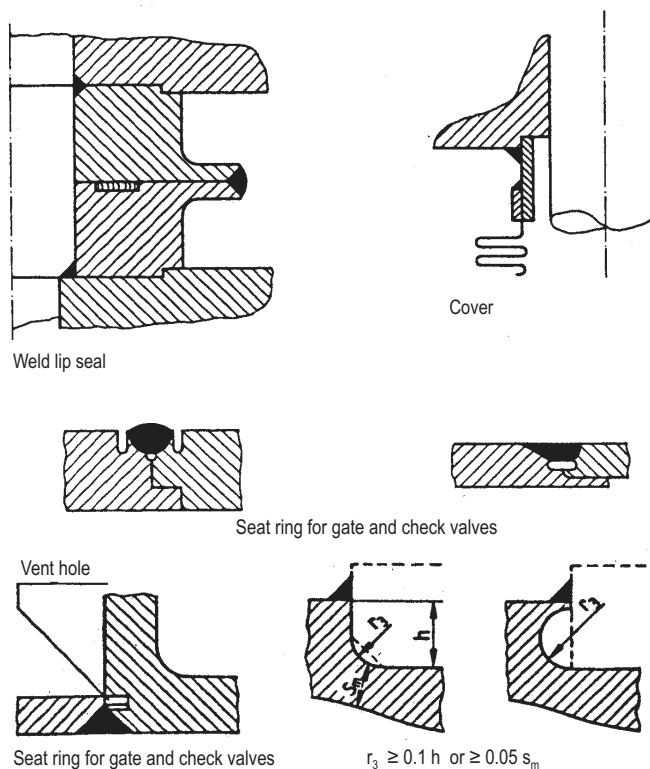
Figure 5.2-3: Examples of welds primarily having sealing function
