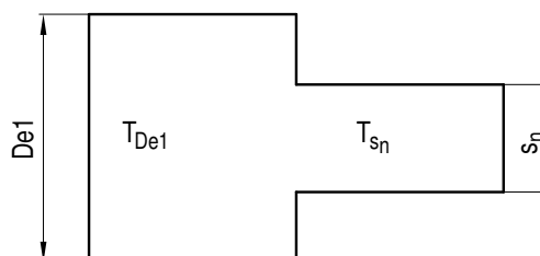
Figure 8.4-6: Determination of \Delta T'
