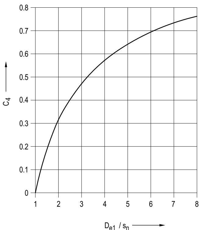
Figure 8.4-11: Maximum magnitude C_4 of the difference in average wall temperatures for wall thicknesses D_{e1} and s_n , resulting from a step change in fluid temperature \Delta T_f
