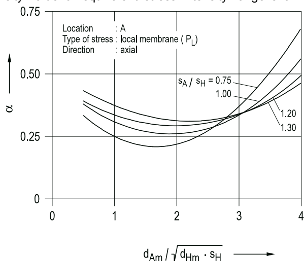
Figure 8.2-4: Stress index \alpha for nozzle in cylindrical shell subject to internal pressure
