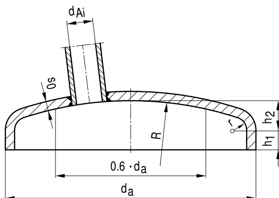
Figure A 2.5-3: Dished head with nozzle
