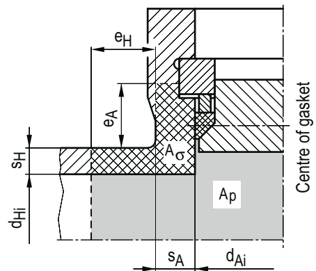
Figure A 4.1-13: Example for cover
