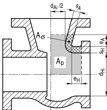
Figure A 4.1-9: Angular-type body
