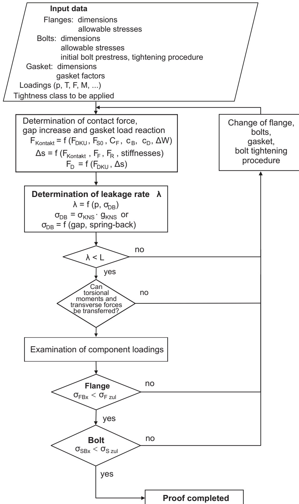
Figure A 2.10-9: Schematic procedural steps for verification of strength of metal-to-metal contact type flanged joints
