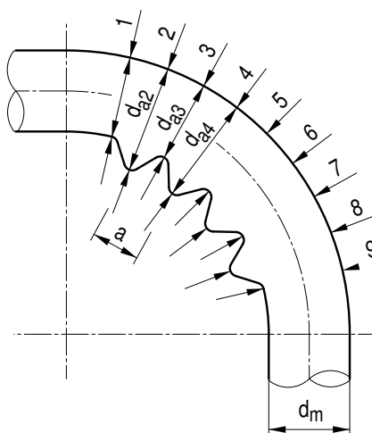
Figure A 5-1: Wrinkles on pipe bend
