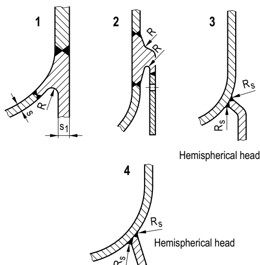
Figure 5.3-5: Examples of component support structures with integral attachment of vertical pressure vessels to bracket supports
