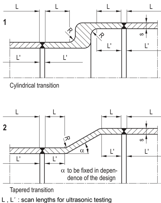
Figure 5.2-5: Examples of allowable configurations of transitions in diameter
