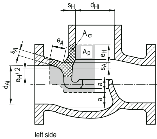
Figure A 4.1-8: Cylindrical valve body
