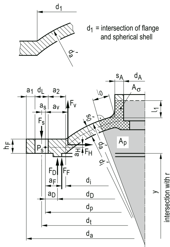
Figure A 2.6-1: Spherically dished head with shallow-dished spherical shell (type I, y > 0 )
