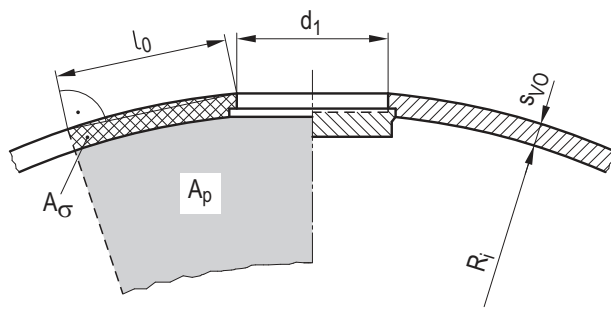
Figure A 2.5-6: Dished head with opening
