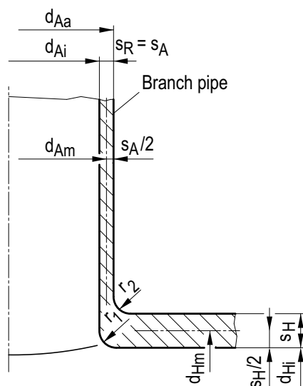
Figure A 5-12: Branch
