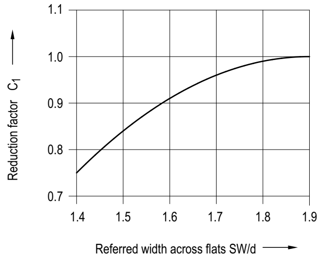
Figure A 2.9-6: Factor C_1 for the reduction of threadstripping resistance of bolt and nut thread due to nut extension
