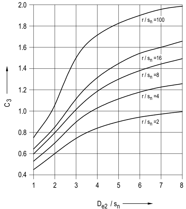
Figure 8.4-8: Stress index for secondary stresses resulting from structural discontinuity due to fluid temperature changes
