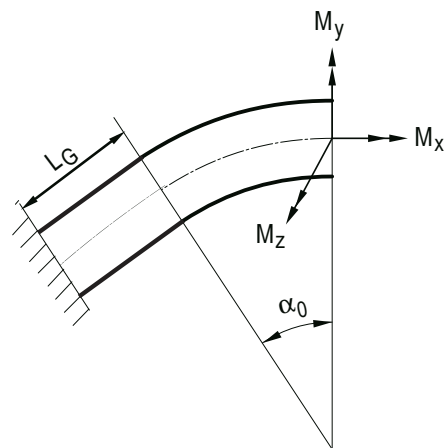
Figure 8.5-9: Direction of moments
