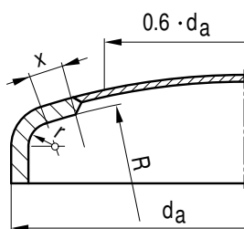
Figure A 2.5-2: Head with differing wall thickness of knuckle and crown section
