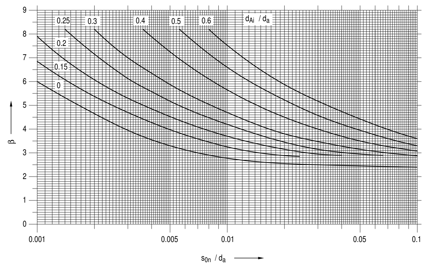
Figure A 2.5-4: Shape factors \beta for torispherical heads
