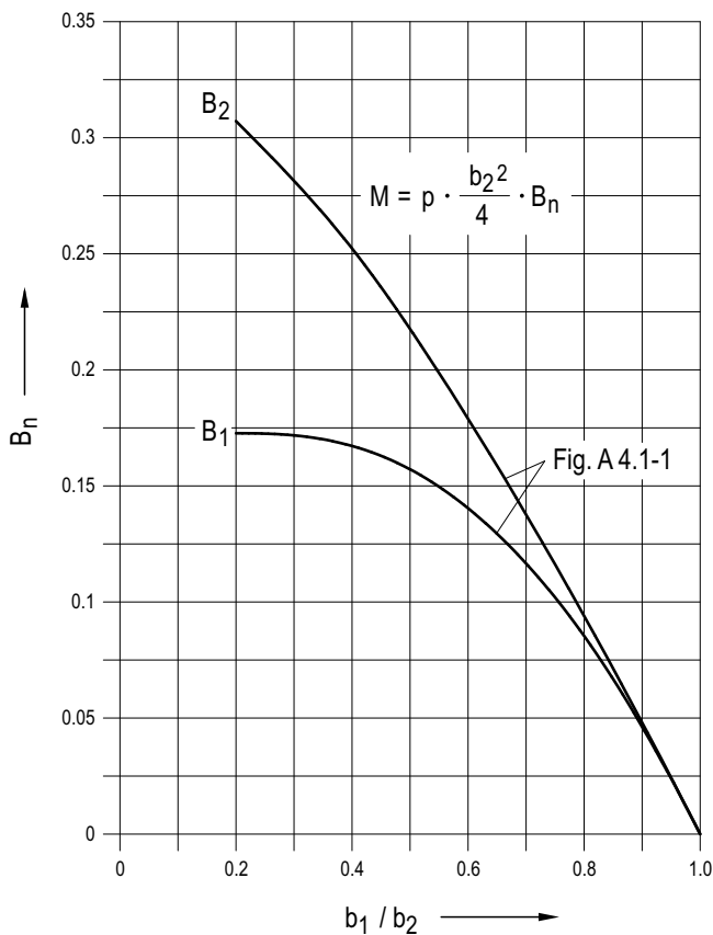
Figure A 4.1-2: Factor B_n for oval cross-sections
