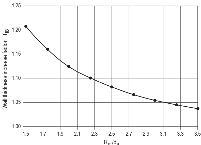
Figure 8.5-1: Wall thickness increase factor for f_{IB} for standard induction bends
