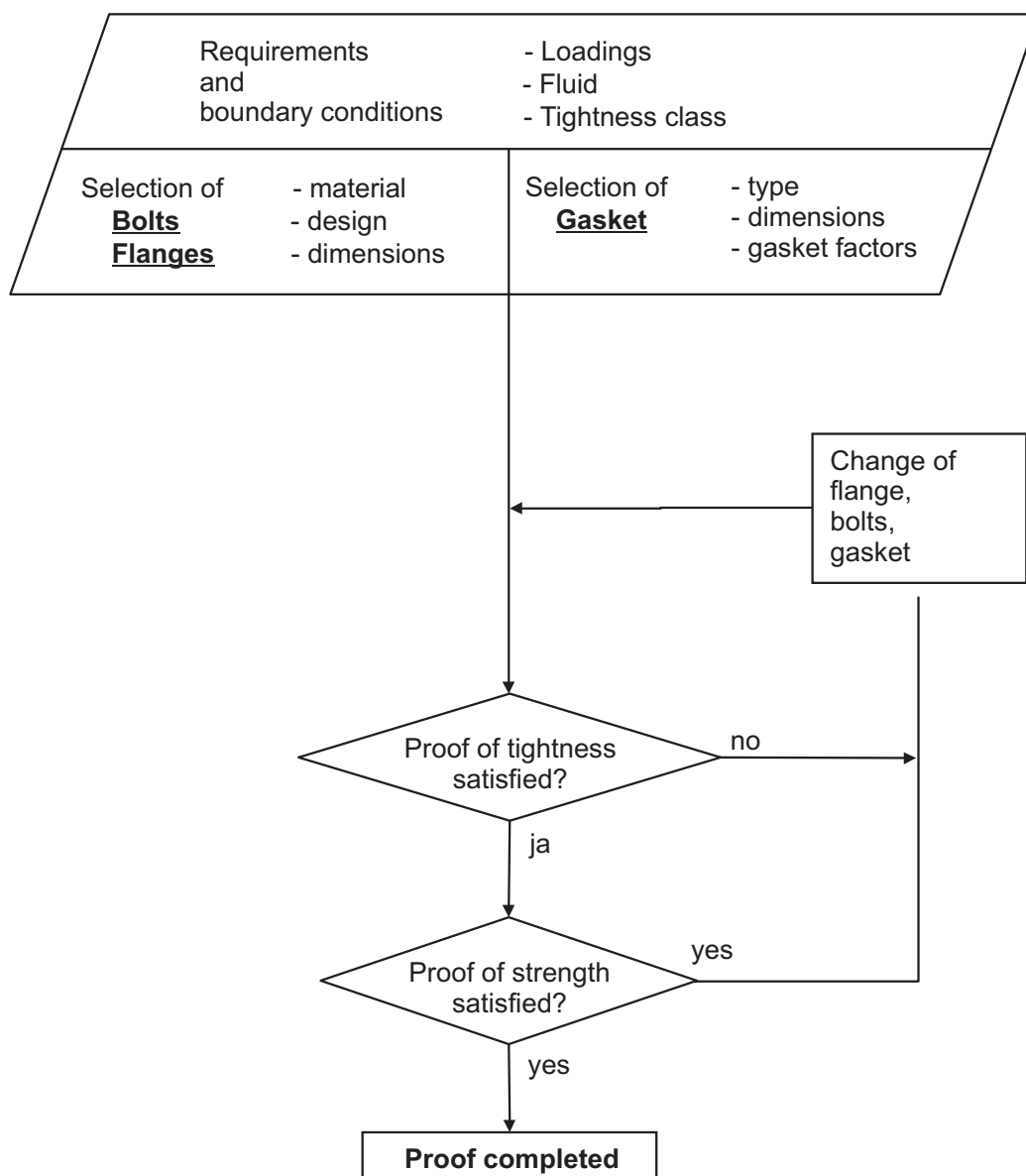
Figure A 2.9-2: General flow diagram for flange design
