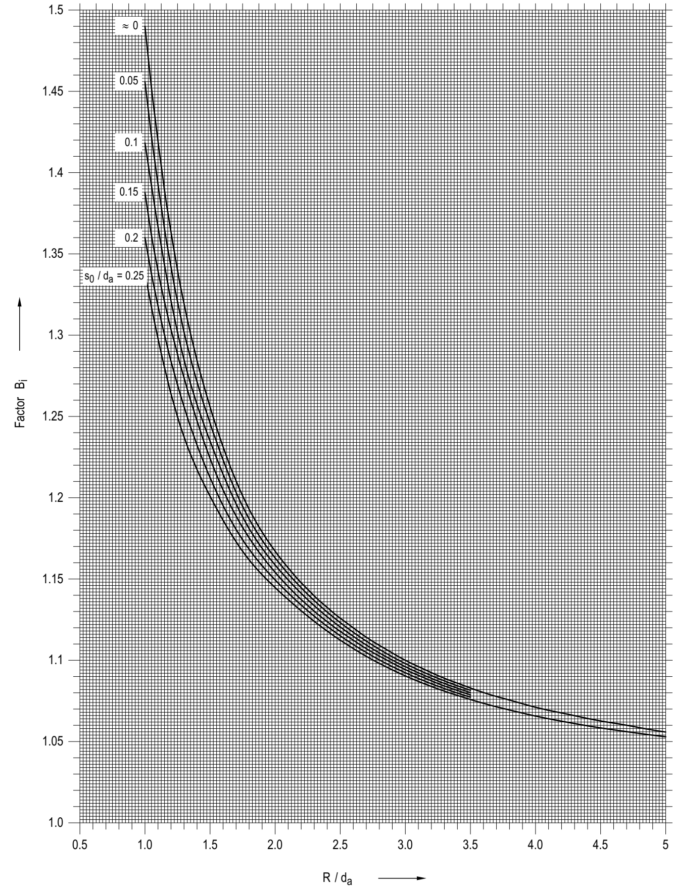
Figure A 5-4: Factor B_i for the intrados at given outside diameter
