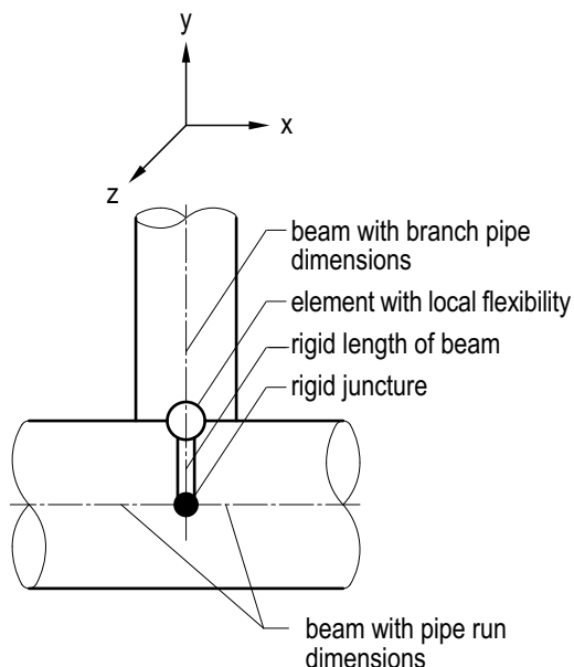
Figure 8.5-10: Modelling of branch connections in straight pipe
