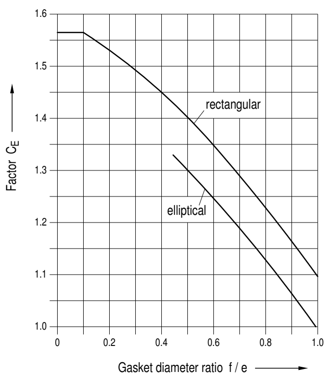
Figure A 2.7-7: Factor C_E for rectangular and elliptical plates
