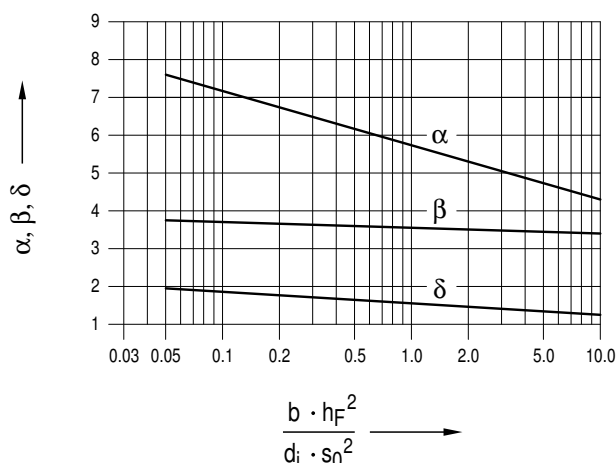
Figure A 2.3-1: Shape factor \beta for the transition flange/spherical shell
