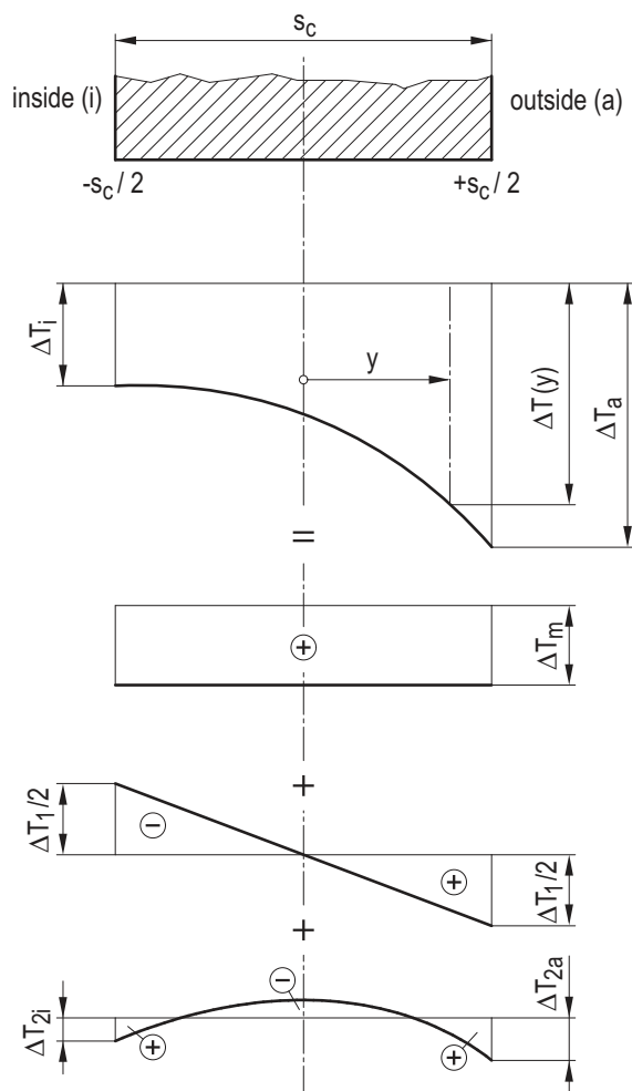
Figure 8.5-2: Decomposition of temperature distribution range
