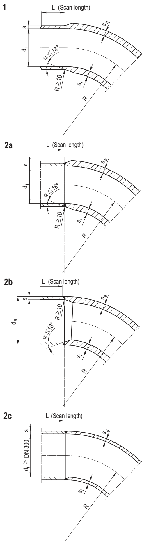
Figure 5.3-3: Design of pipe bends
