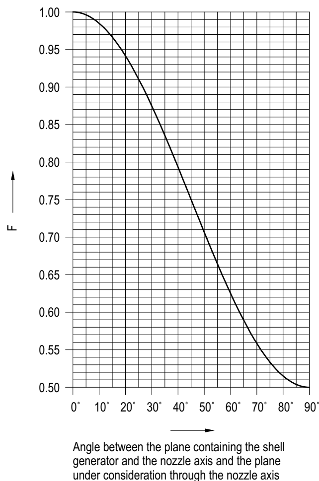
Figure A 2.8-1: Chart for determining the correction factor F for nozzles normal to cylindrical or conical shells
