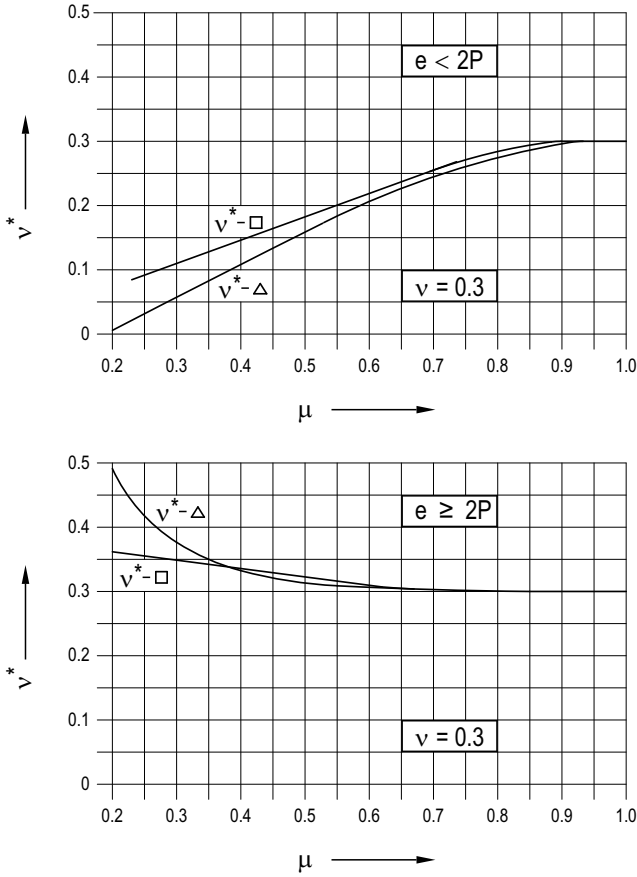
Figure 8.2-15: Effective elastic constants of perforated plate
