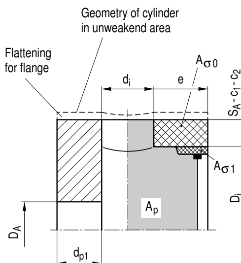
Figure A 3.3-4: Design sketch for an annular casing with flattening and opening; the gasket lies on the inside of the cylinder
