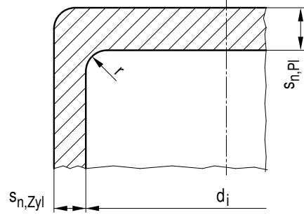
Figure A 2.7-1: Flat plate integral with cylindrical section (for design see Figure 5.2-7)
