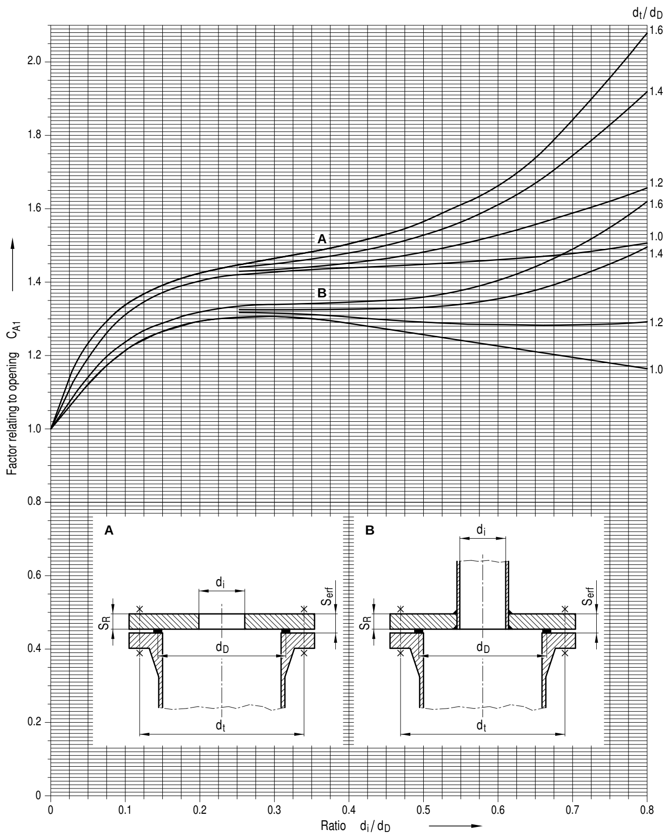
Figure A 2.7-4: Factor C_{A1} for unstayed circular plates with opening and additional edge moment
