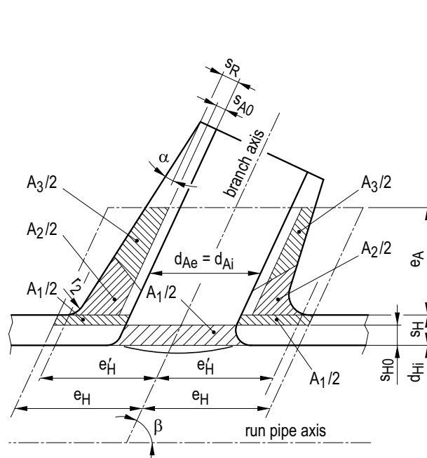
Figure A 2.8-9: Oblique conical branch
