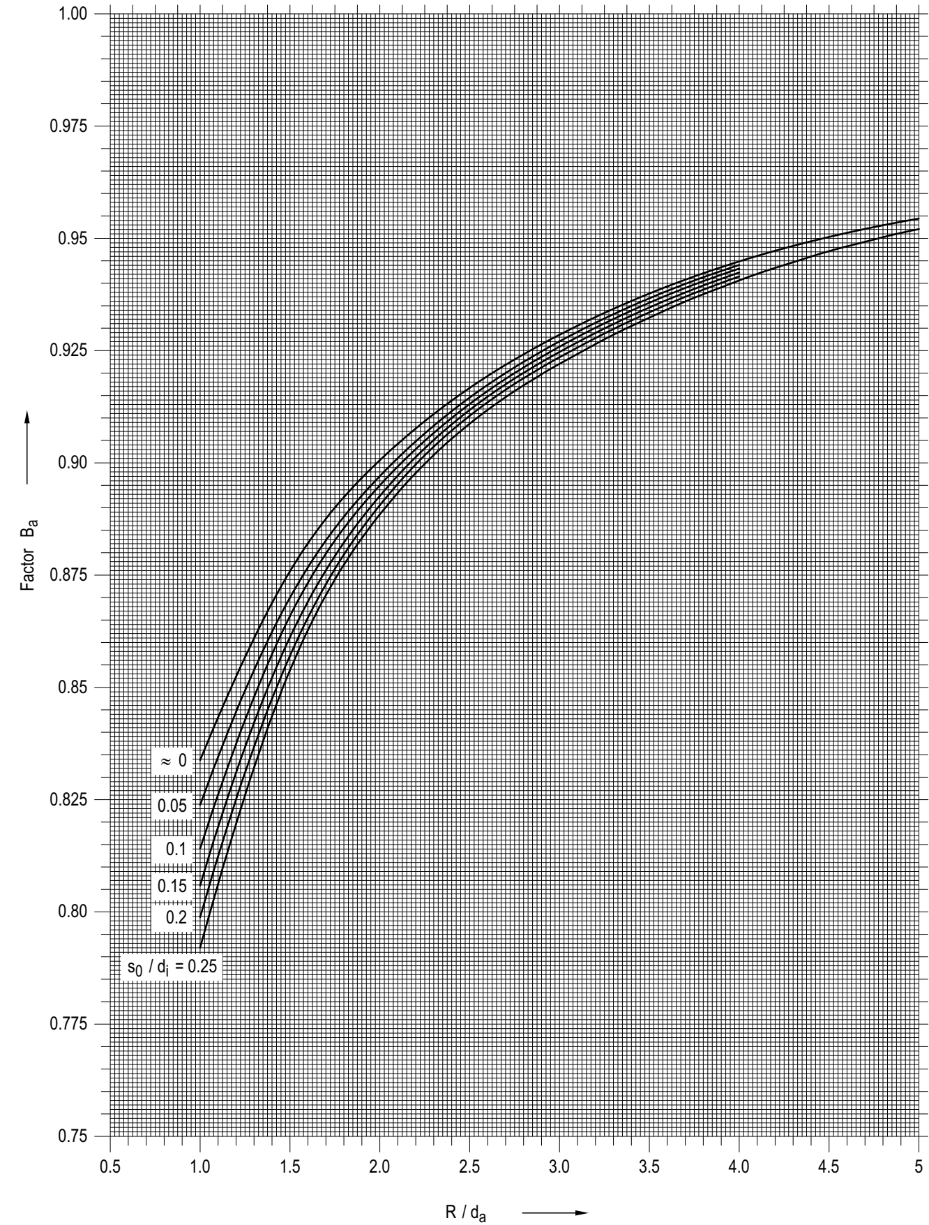
Figure A 5-6: Factor B_a for the extrados at given outside diameter
