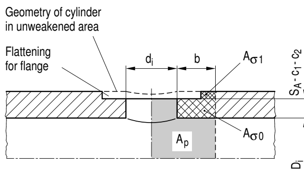
Figure A 3.3-1: Design sketch for barrel-type casings and adjacent openings in longitudinal direction of cylinder
