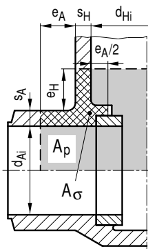
Figure A 4.1-10: Valve body
