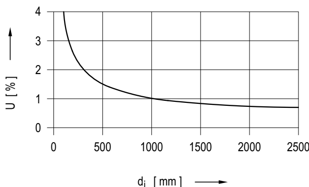
Figure 7.1-3: Ovalities
