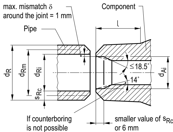
Figure 8.5-5: Concentric reducer
