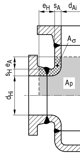
Figure A 4.1-12: Valve body
