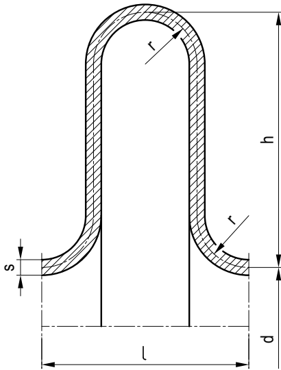
Figure 8.2-12: Parallel-sidewall convolution of bellows expansion joint
