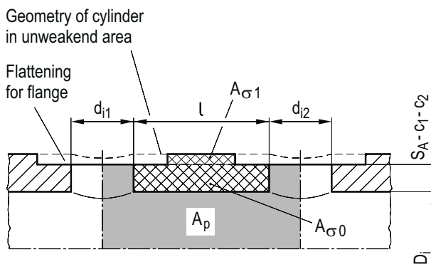
Figure A 3.3-2: Design sketch for barrel-type casing with flattening and adjacent openings in longitudinal direction of cylinder
