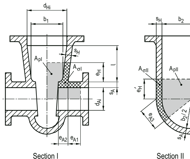
Figure A 4.1-6: Valve bodies
