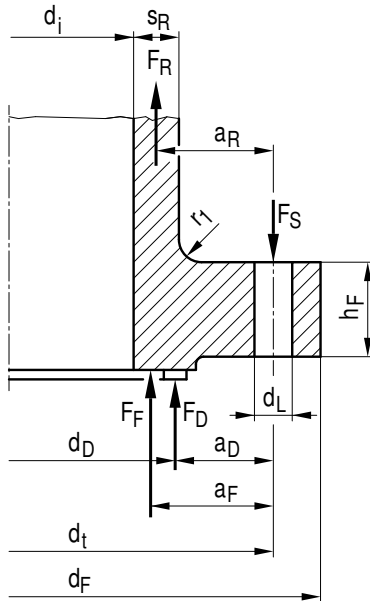
Figure A 2.10-4: Welding-neck flange with cylindrical hub
