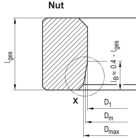
Figure A 2.9-5: Representation of design values for the nut (with tapered portion)
