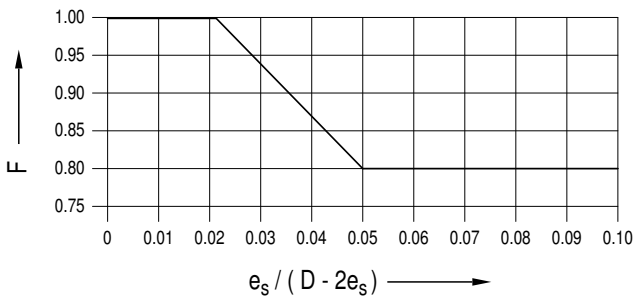
Figure 8.2-17: Determination of F-values
