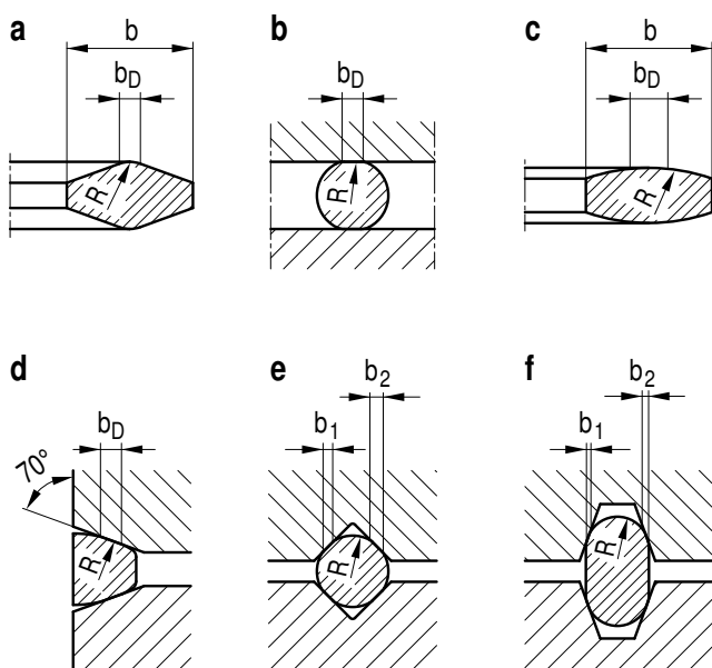
Figure A 2.11-3: Gasket profiles for metallic gaskets with curved surfaces
