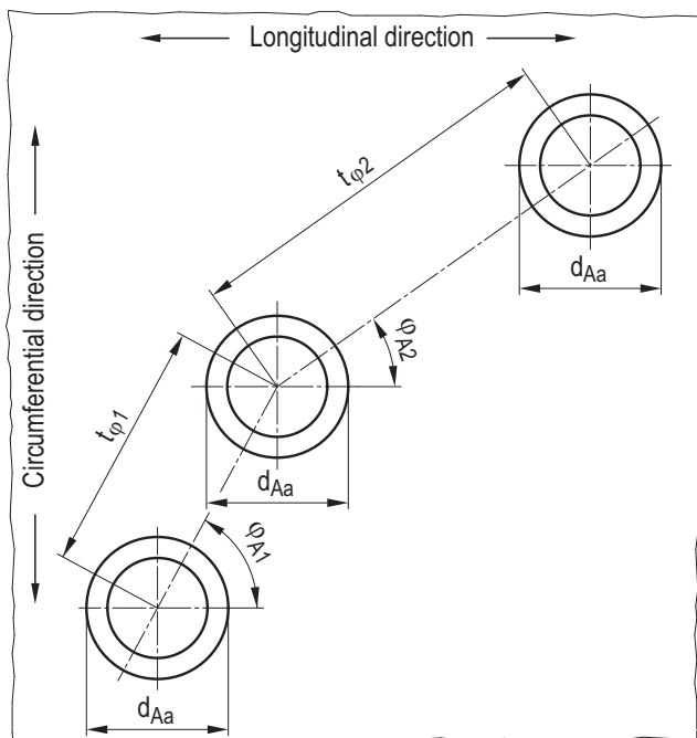
Figure A 5-17: Adjacent openings with different centre-to-centre distances (shown as developed length)
