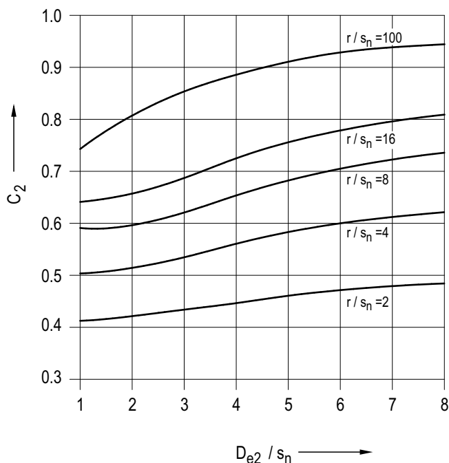
Figure 8.4-10: Stress index C_2 for secondary thermal stresses resulting from structural discontinuity
