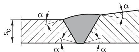
Figure 8.5-3: Allowable weld contour
