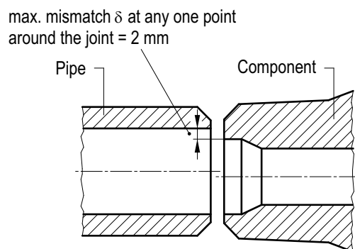
Figure 8.5-4: Butt weld alignment and mismatch tolerances for unequal inside diameter and outside diameter when fairing or back welding on the inside is not possible
