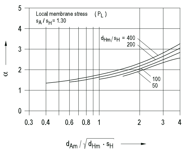
Figure 8.2-10: Stress index \alpha for nozzle in spherical shell subject to internal pressure for P_L
