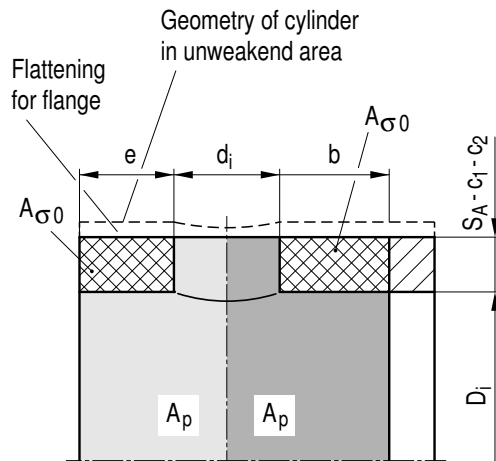
Figure A 3.3-5: Design sketch for pipe casing with flattening and opening
