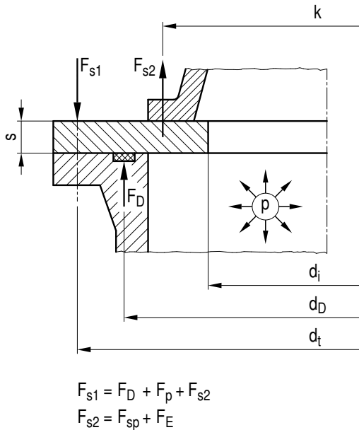
Figure A 2.7-11: Body cover with opening for stem, without reinforcement of opening
