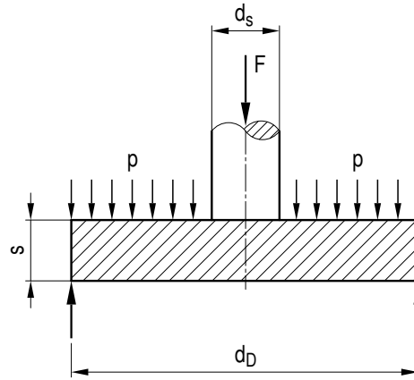
Figure A 2.7-14: Valve sealing disk in the form of a circular plate
