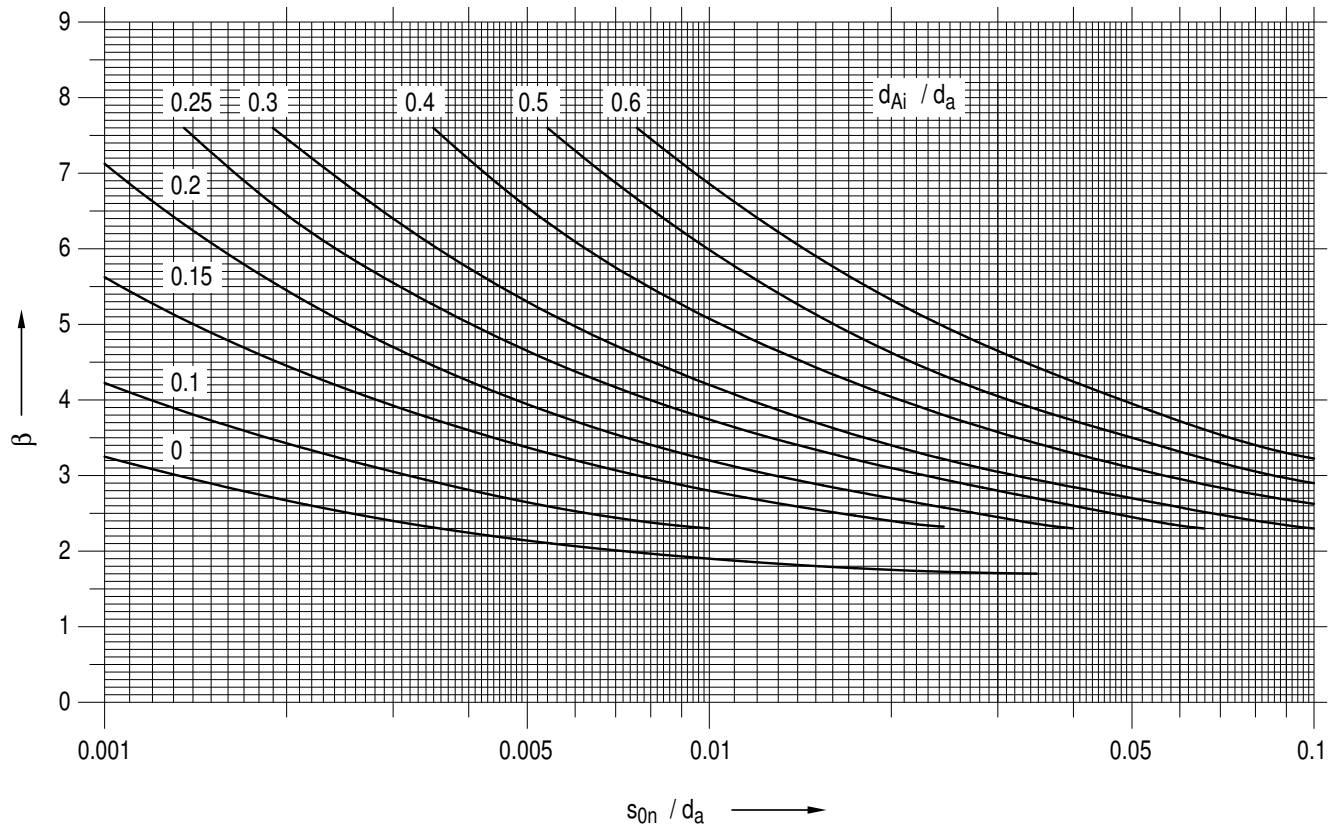
Figure A 2.5-5: Shape factors \beta for semi-ellipsoidal heads
