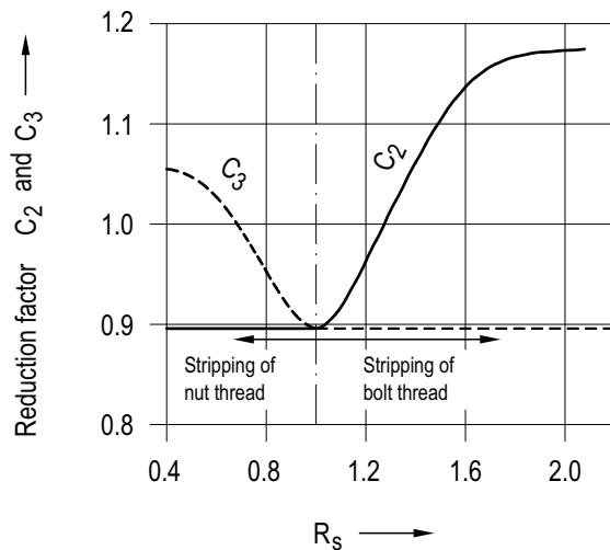
Figure A 2.9-7: Factor for reduction of threadstripping resistance of bolt and nut thread due to plastic deformation of thread
