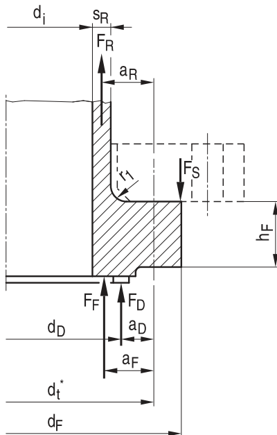
Figure A 2.10-5: Welding stub with cylindrical hub
