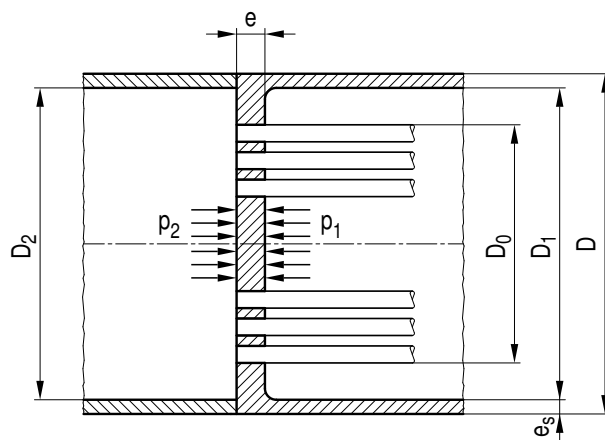
Representation of geometric relationship in the heat exchanger tubesheet area
