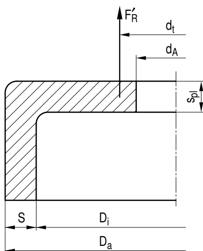
Figure A 3.3-8: Transitional area from cylinder to flat head
