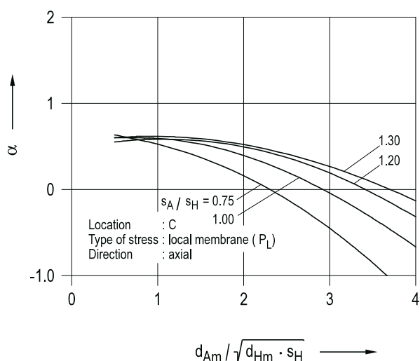
Figure 8.2-5: Stress index \alpha for nozzle in cylindrical shell subject to internal pressure
