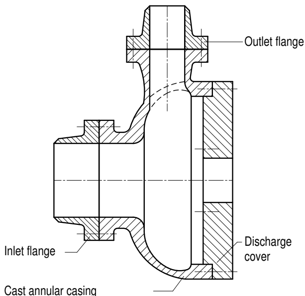
Figure A 3.2-2: Example of a single-stage annular casing pump with cast
