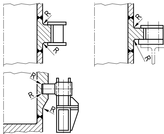
Figure 5.3-7: Examples of component support structures of vertical vessels with forged rings
