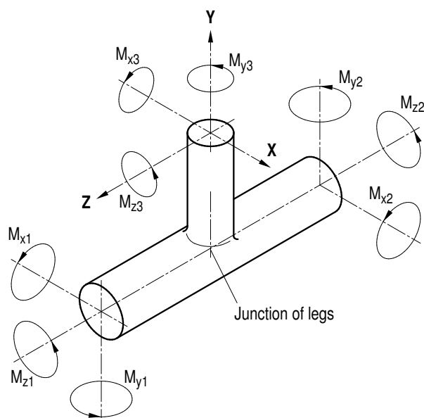
Figure 8.5-11: Moments on tee
