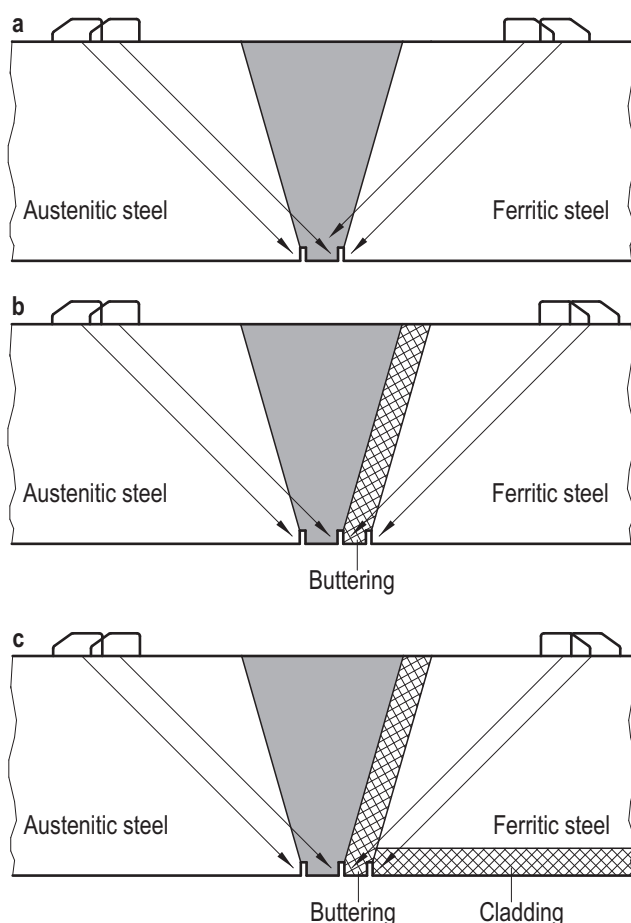
Figure 4-2: Location of notches and sound beam directions for the test for longitudinal defects of welded joints between ferritic and austenitic steels
