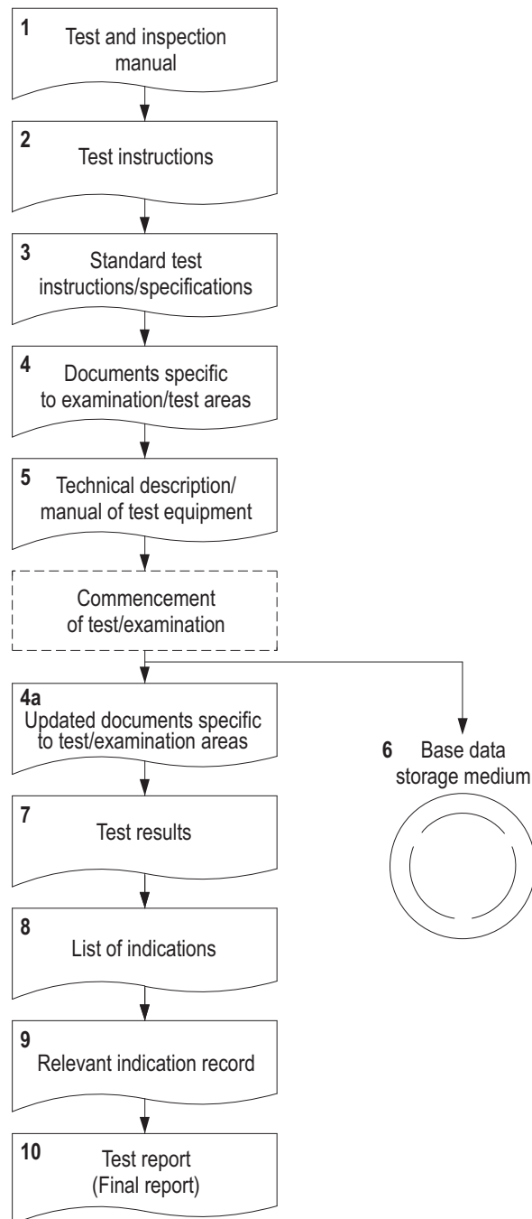
Figure 11-1: Documents for the documentation of automated ultrasonic in-service tests
