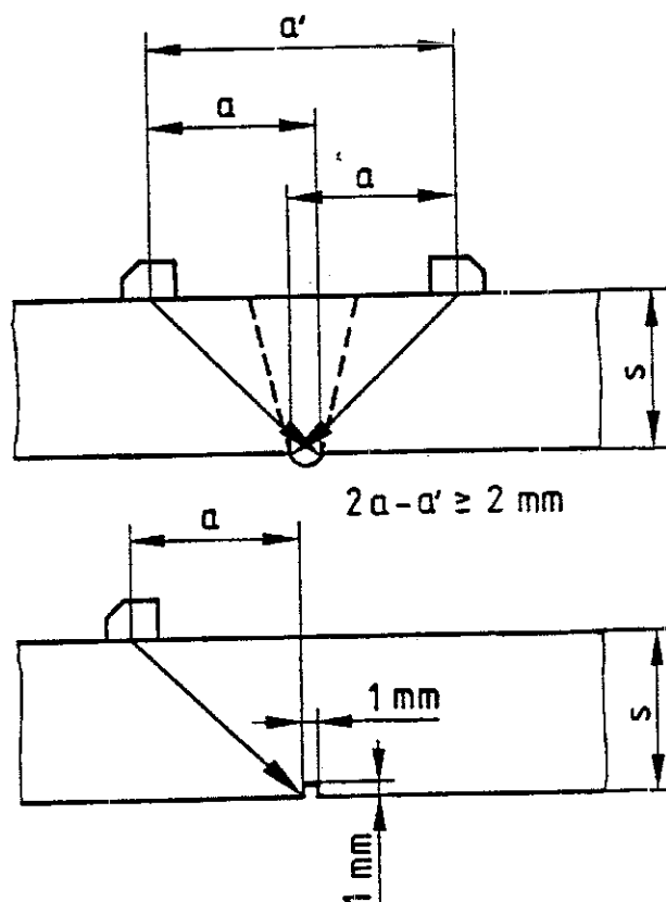
Figure B-12: Demonstration of shape-related indications from the root region of seams welded from only one side
