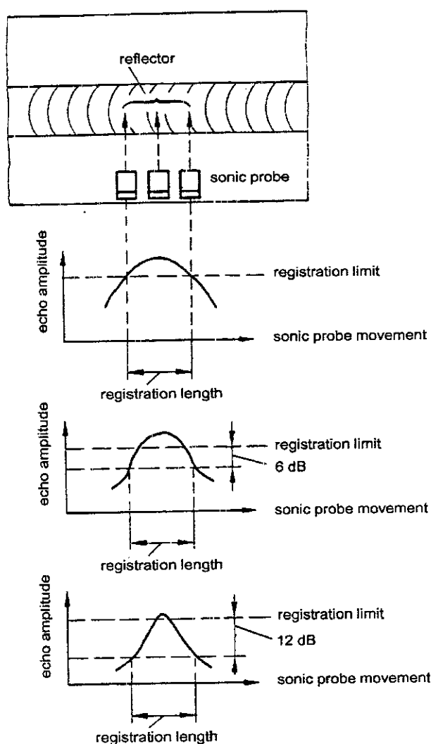
Figure B-10: Determination of the registration length
