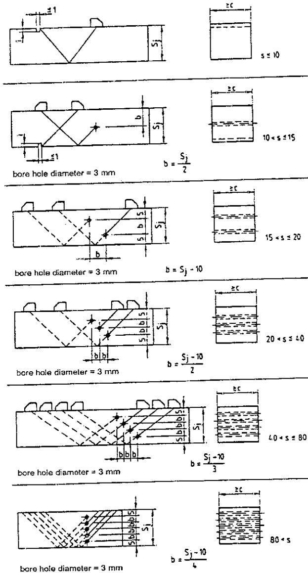
Figure B-1: Reference bodies for the sensitivity adjustments of the angle beam examination
