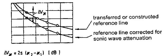
Figure B-9: Accounting for sonic wave attenuation by the reference line method for the case of \kappa_2 > \kappa_1
