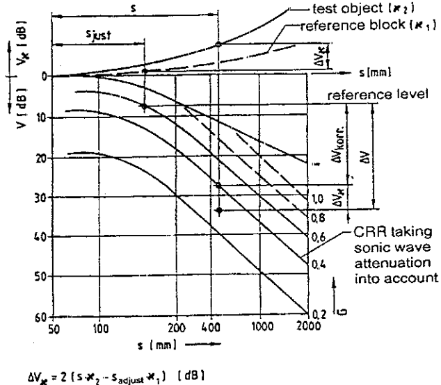
Figure B-8: Accounting for sonic wave attenuation in the DGS diagram for the case of \kappa_2 > \kappa_1
