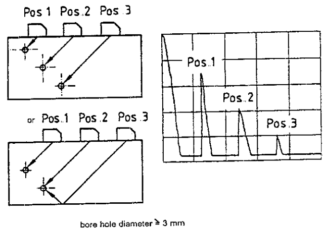
Figure B-3: Creation of indications from transverse bore hole in various distances
