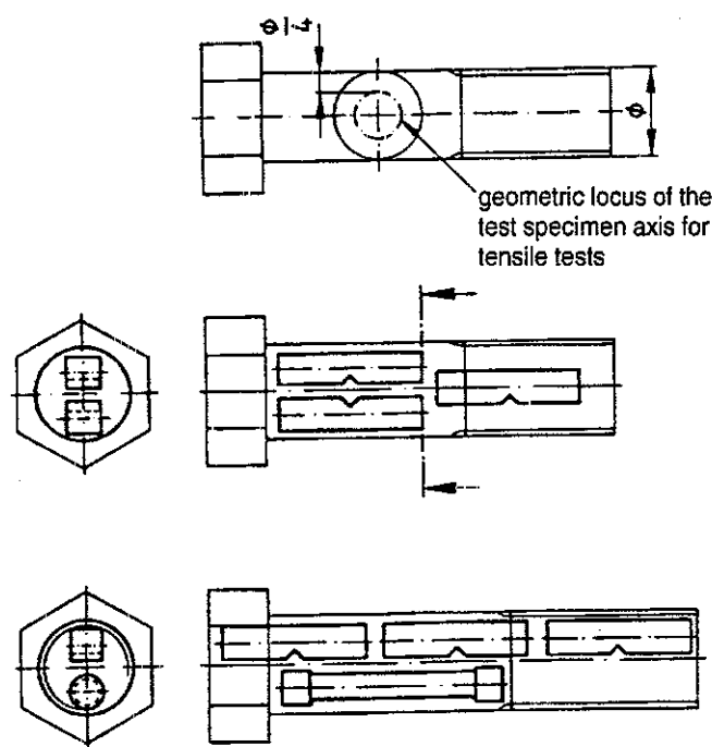
Figure 9-1: Specimen removal from bolt blanks with hot formed bolt head and subjected to subsequent quenching and tempering
