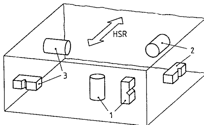
Figure 3-1: Identification of the orientation of test specimens of flat product forms
