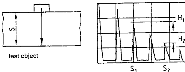
Figure B-5: Determination of the transfer correction for the straight-beam or angle-beam examination with a single or double V sonic path
