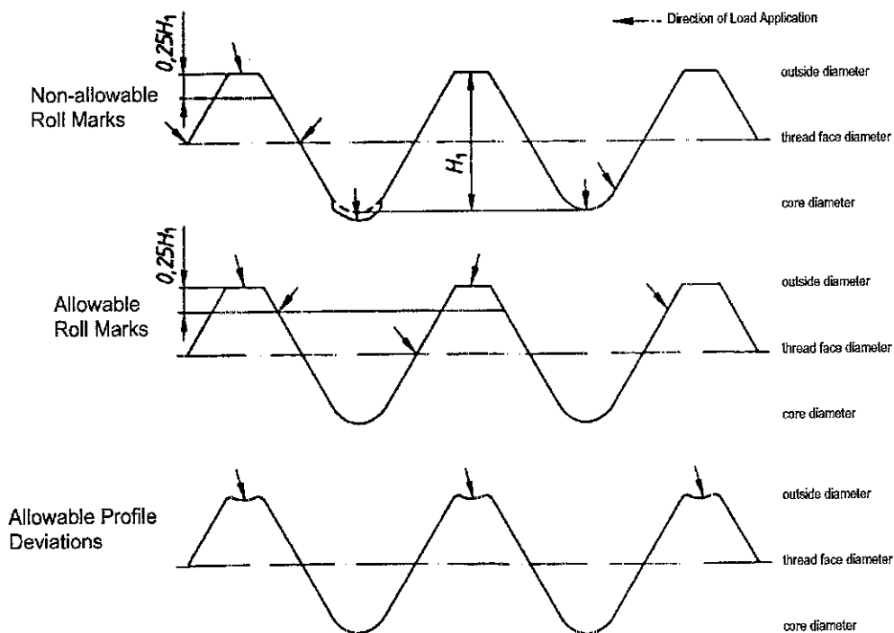
Figure 8-1: Appearance, shapes and locations of flaws in bolts and nuts
