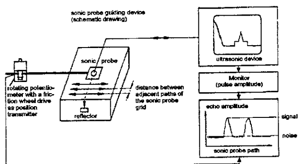
Figure B-11: Measurement device for employing focussing sonic probes for the determining the reflector size
