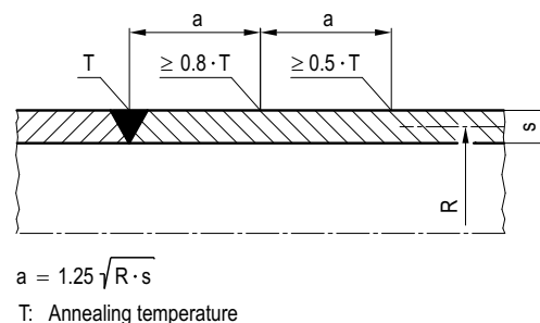
Figure B 4-1: Temperature pattern during stress relieving
