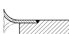
Detail A Design type 2 for single-ply and multi-ply bellows 2)
