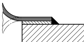
Detail A Design type 5 for multi-ply bellows 2) 3)
