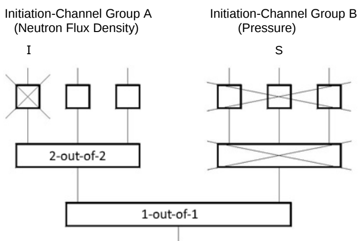
Figure 4-6: Schematic where a common-mode failure occurs in Initiation-Channel Group B during the repair of an initiation channel in Initiation-Channel Group A. The design-basis accident is covered by Initiation-Channel Group A (2-out-of-2).
