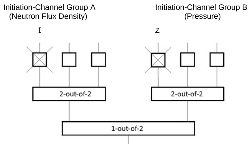
Figure 4-4: Schematic where one initiation channel in Initiation-Channel Group A is inoperable due to repair and a random failure occurs in Initiation-Channel Group B. The design-basis accident is covered by Initiation-Channel Group A (2-out-of-2) and by Initiation-Channel Group B (2-out-of-2).
