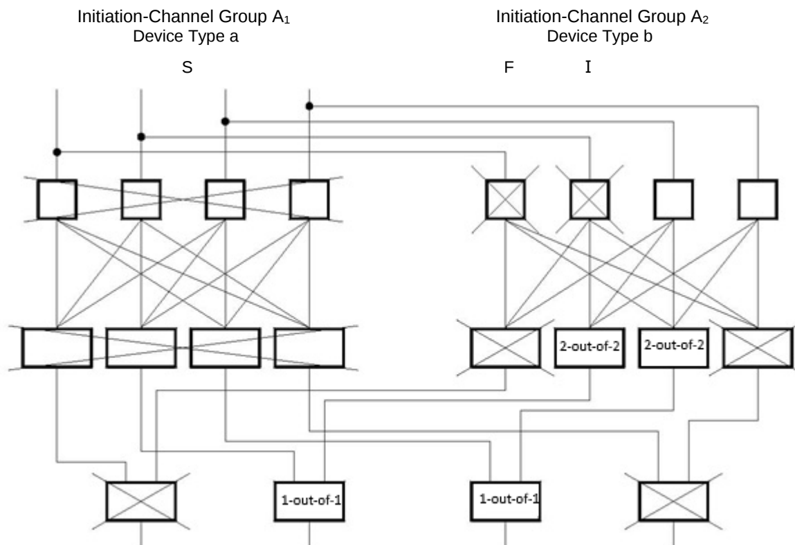
Figure 4-9: Schematic showing how the situation shown in Figure 4-8 may develop in case of the most unfavorable failure combination: During repair of one initiation channel in Initiation-Channel Group A 1 , a common-mode failure occurs in the Device Type a. Additionally, one actuation channel in Initiation-Channel Group A 2 becomes inoperative due to a secondary failure. The design-basis accident is sufficiently covered by actuating two of the 50 % subunits of the safety system.
