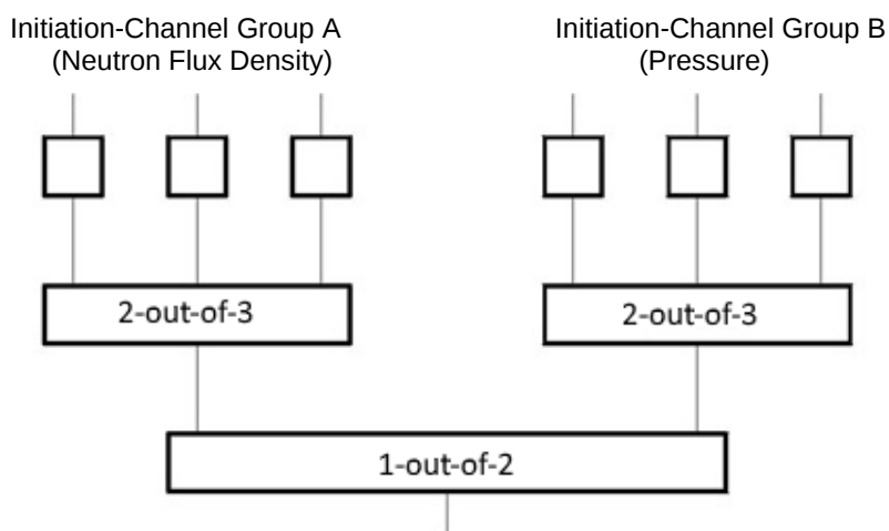
Figure 4-2: A possible schematic for the actuation of the reactor scram; it is caused by reactivity disturbances where two actuation criteria derived from different process variables (e.g., neutron flux density and pressure) are available and any secondary failures in data acquisition can be precluded.
