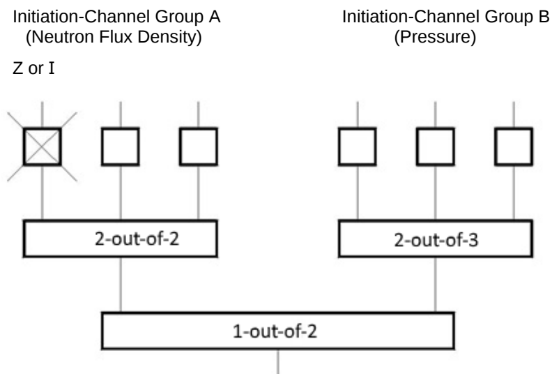
Figure 4-3: Schematic where one initiation channel of Initiation-Channel Group A is inoperable because of maintenance or due to the failure of one initiation channel caused by a single random failure. The design-basis accident is covered at least by Initiation-Channel Group A (2-out-of-2) and Initiation-Channel Group B (2-out-of-3).
