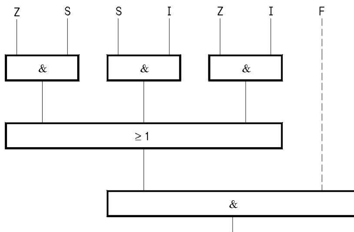
Figure 4-1: Failure combinations to be applied
