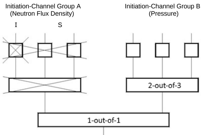
Figure 4-7: Schematic where, during repair of one initiation channel in Initiation-Channel Group A, a common-mode failure occurs in the same initiation-channel group. The design-basis accident is covered by Initiation-Channel Group B (2-out-of-3).
