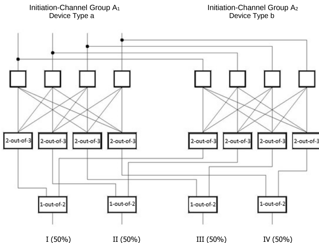
Figure 4.8: Schematic showing the basic layout for the actuation of the fourfold mutually redundant 50 % subunits of the safety system in case of a design-basis accident where only a single safety variable is available and where secondary failures in data acquisition (e.g., a break in the differential pressure line) must be assumed as physically possible and as not being actuation oriented. The devices for data acquisition up to and including the measuring transducers in the two initiation-channel groups are of diverse types (Device Type a, Device Type b)
