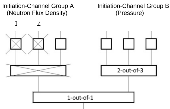
Figure 4-5: Schematic where, during the repair of one initiation channel in Initiation-Channel Group A, a random failure occurs in another initiation channel of the same initiation-channel group. The design-basis accident is covered by Initiation-Channel Group B (2-out-of-3).
