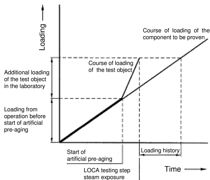
Figure 6-2: Exemplary graph showing the loading history for the proof as specified under Section 6.2.1 para. 3
