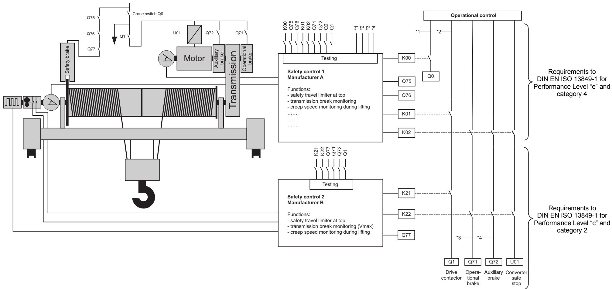
Figure E-4: Example for realization of the requirements specified in Table E-1 for the functions ser. no. 12b "Switch-off in case of excess of allowable speed at hoist end position " ser. no. 31 "Gear box break monitoring with triggering of safety brake" ser. no. 33a "Safety travel limiter in lift direction" in lifting equipment according to sections 4.3 or 4.4 (Example of hoist with single drive mechanism chain and insufficient travel stop path upon response of the safety travel limiter in the main circuit, in lift direction)
