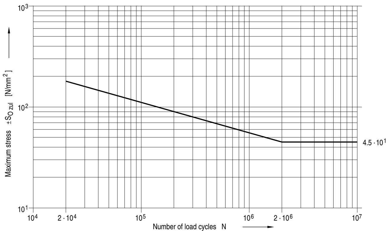
Figure C-10: S/N diagram for notch case K 4 according to DIN 15018-1, R = 0
