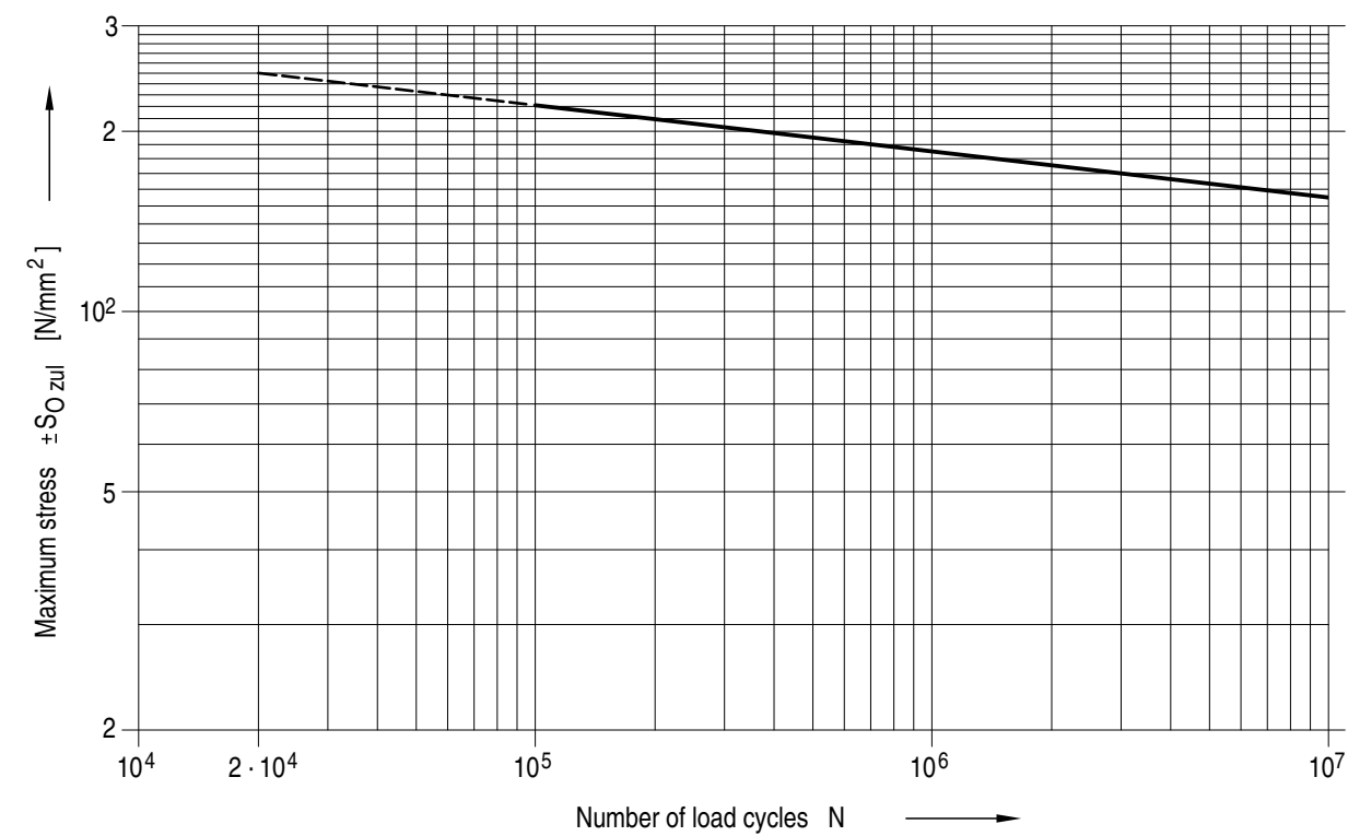
Figure D-5: S/N diagram for notch case K 1 (single-vee butt weld), R = 0
