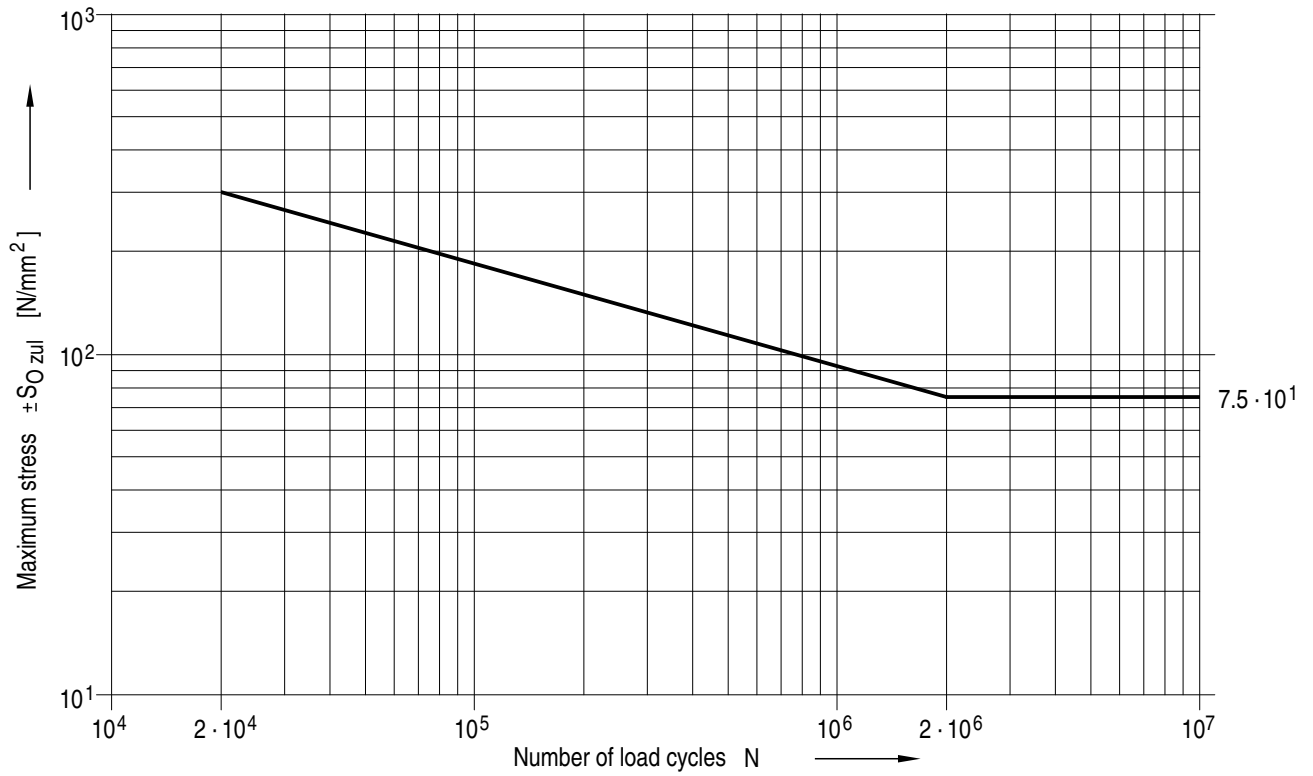
Figure C-9: S/N diagram for notch case K 3 according to DIN 15018-1, R = 0
