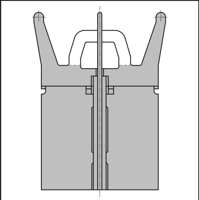
Fig. C-12: Control rod head for BWR
