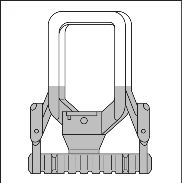
Fig. C-11: Fuel assembly head for BWR
