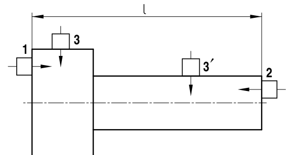
Figure B-3: Scanning positions for stepped bolts and trunnions (example)
