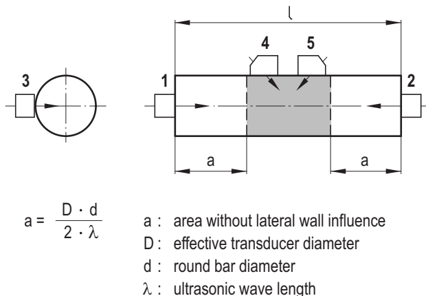
Figure B-1: Scanning positions for round bars
