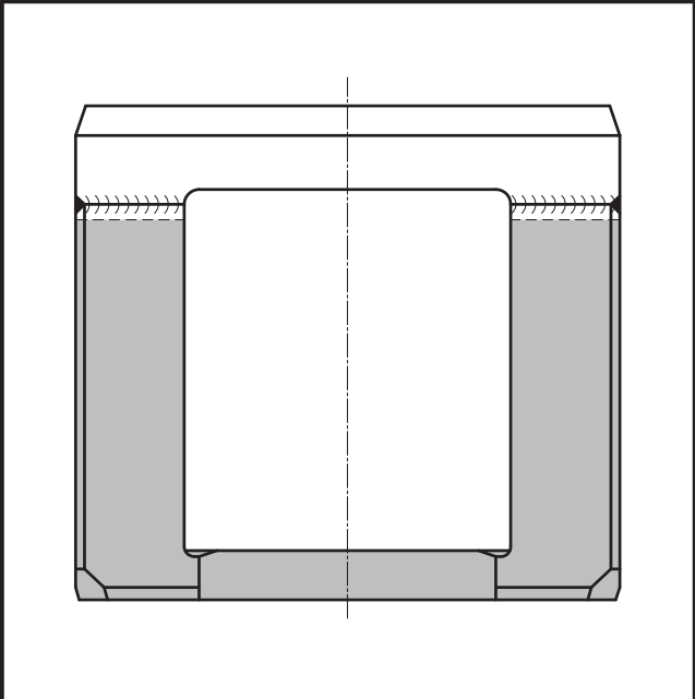
Fig. C-9: Fuel assembly head for PWR
