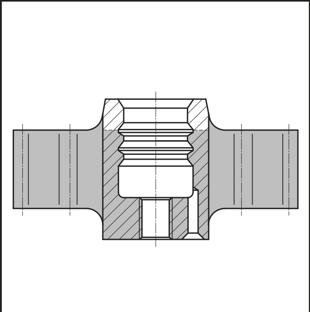
Fig. C-10: Control rod spider for PWR
